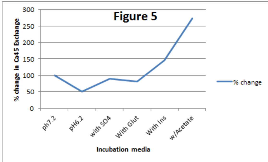
Figure 5. Percentage change of Ca 45 exchange rates
