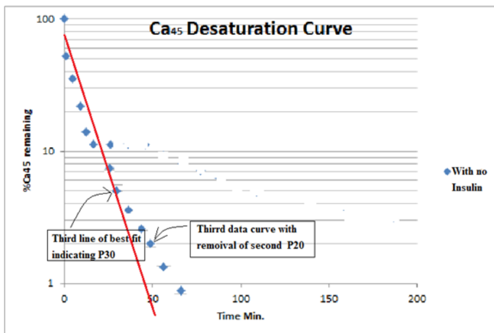
Figure 3. Step three in determining the curvilinear line of best for the multi term exponential curve for the experimental data set
