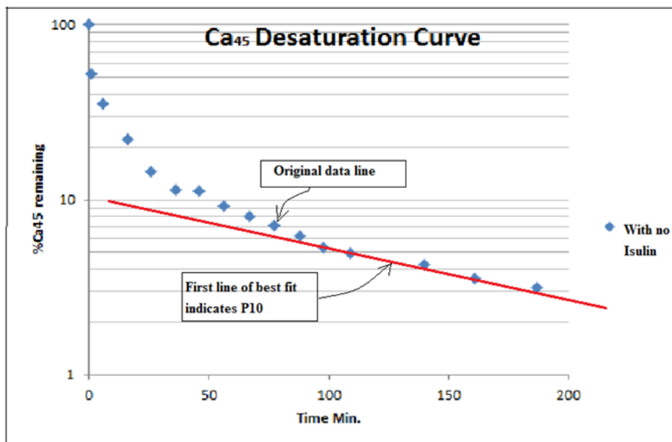
Figure 1. Step one in determining the curvilinear line of best for the multi term exponential curve for the experimental data set
