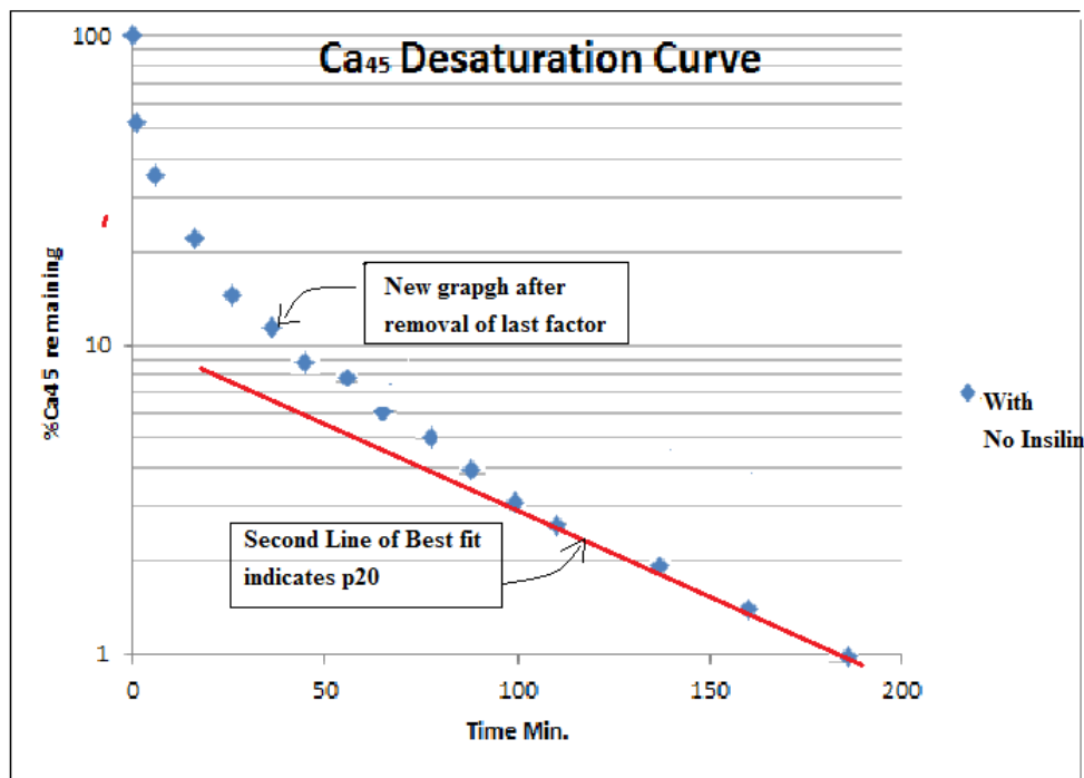
Figure 2. Step two in determining the curvilinear line of best for the multi term exponential curve for the experimental data set
