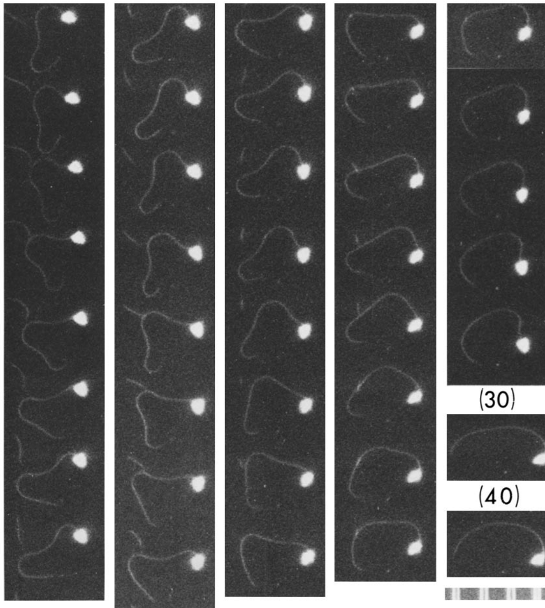
FIGURE 9 Movement of a sea urchin spermatozoon during exposure to \text{CO}_2 in a reactivation solution at \text{pCa} = 4 , after demembration in the presence of 2 \text{ mM CaCl}_2 . The exact time course of exposure to \text{CO}_2 was not recorded, but the first effects can probably be detected during the second beat cycle shown here (the second vertical strip). The flash frequency was 60 \text{ Hz} ; the scale divisions are 10 \mu\text{m} ; and the numbers above the last two frames indicate the number of frames omitted.
