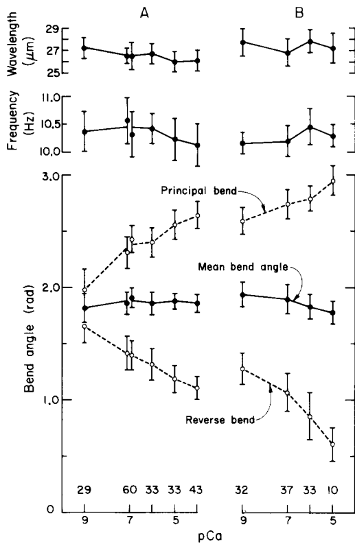
FIGURE 1 Effect of \text{Ca}^{2+} concentration on parameters of movement of demembrated flagella. Results for spermatozoa demembrated with Triton solutions containing 2 mM \text{CaCl}_2 are shown in A; results for spermatozoa demembrated with Triton solutions without \text{CaCl}_2 are shown in B. Results were obtained with two different sperm samples, which gave significantly different degrees of asymmetry. The values shown are the mean values for the means and standard deviations obtained with each sperm sample. The total number of spermatozoa measured at each \text{Ca}^{2+} concentration is indicated at the bottom of the figure. In A, the points at \text{pCa} = 7 represent results obtained with reactivation solutions containing 2 mM EGTA, on the left, and 2 mM EDTA, on the right. ( \text{pCa} indicates a \text{Ca}^{2+} concentration of 10^{-\text{pCa}} M.)
