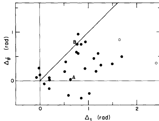
FIGURE 6 Values of the two components of flagellar asymmetry, \Delta_{\dot{\theta}} and \Delta_t , defined in the text. Point B corresponds to the flagellum shown in Figs. 2 and 3. The two open circles correspond to flagella showing more extreme asymmetry, involving a decrease in the reverse bend angle; the point at the far right corresponds to the flagellum shown in Figs. 7 and 8.
