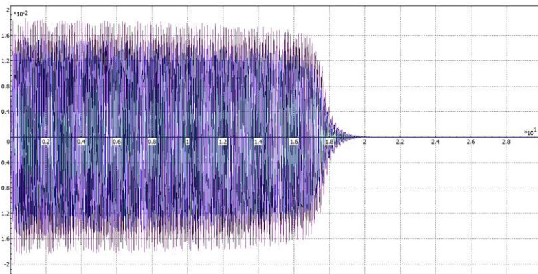
Fig. 6. Horizontal lateral displacement of wheelsets (DMetI wheel profile). Horizontal axis: time [s], Vertical axis: wheelset lateral displacement [m]
