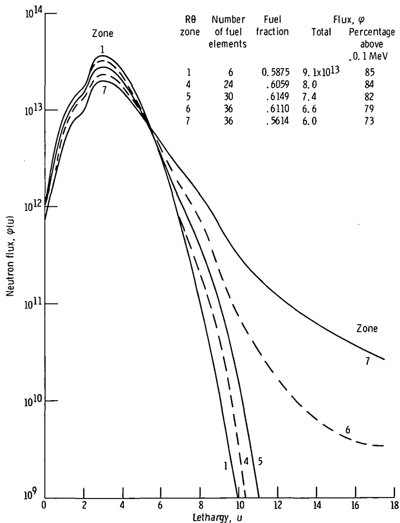
Figure 7. - Zone spectra from R \theta calculations. Power normalized flux, 1.575 thermal megawatts.
