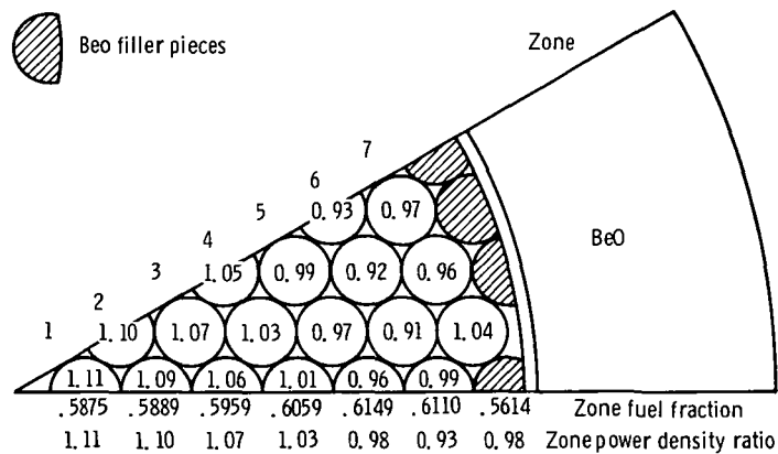
Figure 4. - Fuel pin and fuel zone power relative to average in R\theta calculations for center traverse. Multiplication factor, 1.057.
