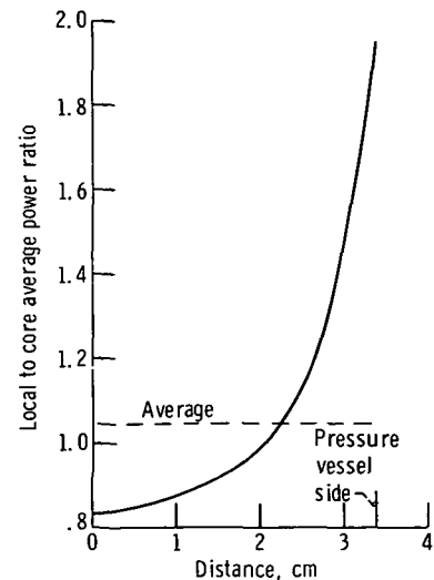
Figure 6. - Fuel pin cell nearest to pressure vessel. Fuel fraction, 0.5614.
