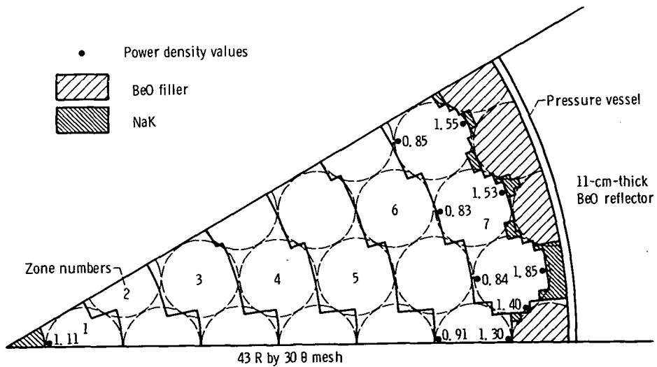
Figure 2. - Rθ calculation model for reference thermionic reactor.
