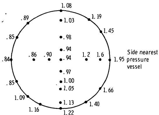
Figure 5. - Fuel cell relative power distribution at selected points. Cell average power density ratio, P/P , 1.04; average power density, \bar{P} , 1.0 for R\theta calculation.
