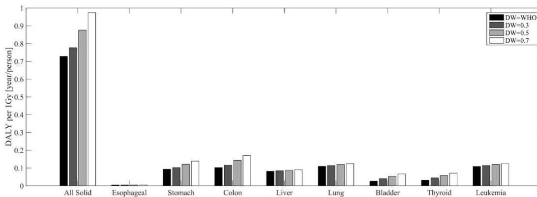
Figure 5. DALY with different DW values (Japanese Men)
