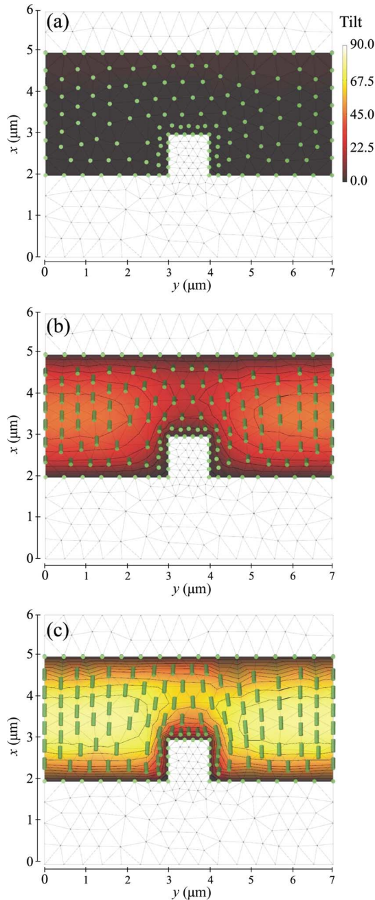
Fig. 5. Orientation of the liquid crystal in a rib waveguide for (a) 0 V, (b) 2 V, and (c) 4 V. The background color indicates the tilt angle of the director as denoted by the colorbar.
