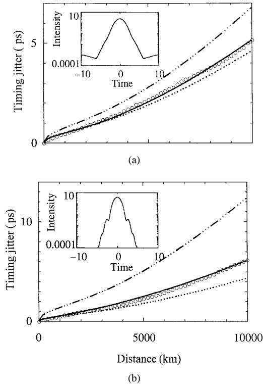
Fig. 1. The root-mean-square central time of the pulse versus distance for a dispersion-managed soliton system. Inserted graphs are intensity profiles of the dispersion-managed solitons plotted on a logarithmic scale. Circles are results of Monte Carlo simulations, solid lines are results of our theory, and the broken lines and dots represent the Gordon–Haus theory and reduced Gordon–Haus theory, respectively; t_{\text{FWHM}} = 20 ps, losses are 0.21 db/km; (a) dispersion coefficients are \beta_1'' = -3.0 ps 2 /km and \beta_2'' = 2.8 ps 2 /km, the amplifier distance is 50 km, amplifiers are placed at the edges and at the midpoints of normal and anomalous dispersion spans, span lengths are L_1 = L_2 = 100 km, peak power at the midpoint of the anomalous dispersion span is 4.12 mW and (b) dispersion coefficients are \beta_1'' = -3.75 ps 2 /km and \beta_2'' = 3.55 ps 2 /km, amplifiers are placed at the edges of the spans, amplifier distance is 100 km, span lengths are L_1 = L_2 = 100 km, peak power at the midpoint of the anomalous span is 1.39 mW. Here, \beta_j'' is the dispersion coefficient and L_j is the length of span j .
