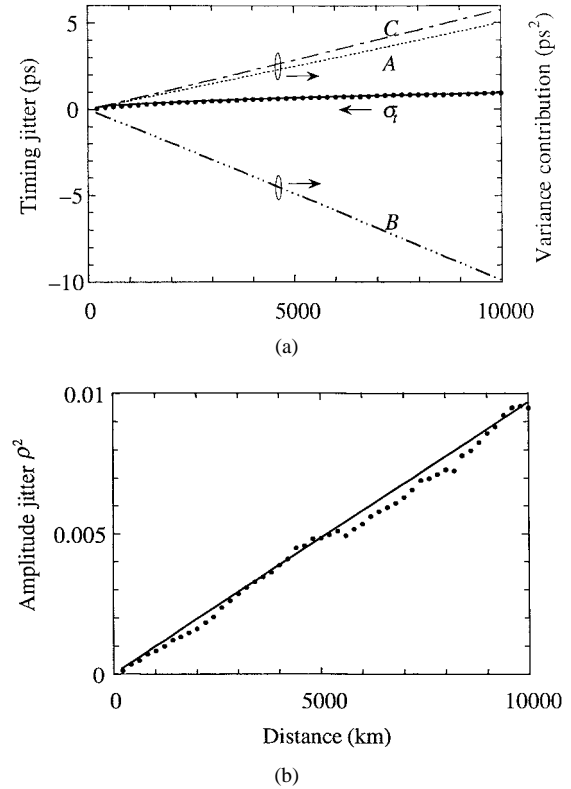
Fig. 2. (a) Timing jitter \sigma_t and (b) amplitude jitter \rho versus distance for a dispersion-managed soliton at zero average dispersion. In (a), we also show the individual contribution of the terms A , B , and C . Solid lines are results of the theory, dots are results of Monte Carlo simulations; the peak power at the midpoint of the anomalous dispersion span is 4.33 mW and t_{\text{FWHM}} = 20 ps, \beta_1'' = -\beta_2'' = -11 ps 2 /km, L_1 = L_2 = 100 km. Amplifiers are placed at the edges and at the midpoints of the spans every 50 km.
