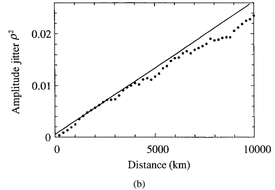
Fig. 7. Plots of the (a) timing jitter \sigma_t and (b) the amplitude jitter \rho versus distance for a 0-1-0 NRZ pulse of 100 ps at zero average dispersion. Fig. 7(a) shows the individual contributions of the terms A , B , and C to the pulse central time variance versus distance. Pulse peak power is 0.35 mW; system parameters are the same that in Fig. 3.
