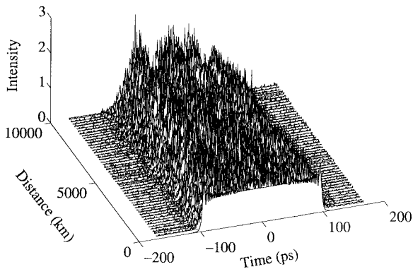
Fig. 10. Evolution of the 0-1-1-0 NRZ pulse in the presence of noise for the system in Fig. 9.
