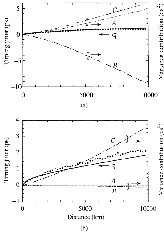
Fig. 3. Dependence of the timing jitter \sigma_t and the contributions of the terms A , B , and C to the central time variance on distance for the dispersion-managed soliton at zero average dispersion in a system with L_1 = L_2 = 50 km, peak power in the midpoint of the anomalous dispersion span of 1.21 mW, amplifier spacing of 50 km and other parameters being the same as in Fig. 2 for the amplifier arrangements at (a) the edges and at (b) the midpoints of the spans.
