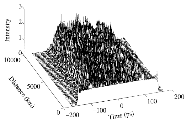
Fig. 12. Evolution of the 0-1-1-1-0 NRZ pulse in the presence of noise for the system in Fig. 11.
