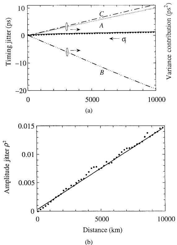
Fig. 5. Plots of the (a) timing jitter \sigma_t and (b) amplitude jitter \rho^2 versus distance for an RZ pulse at zero average dispersion. Fig. 5(a) shows individual contributions of the A , B , and C terms to the pulse position variance versus distance. Solid lines are results of the theory; dots are the results of the Monte Carlo simulations; pulse duration and peak power at the midpoint of the anomalous dispersion span are t_{FWHM} = 20 ps and 1.08 mW, \beta_1' = -\beta_2' = -11 ps 2 /km, L_1 = L_2 = 100 km. Amplifiers are placed at the edges and at the midpoints of the spans every 50 km.
