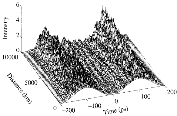
Fig. 6. Evolution of the RZ pulse in the presence of noise for the system in Fig. 5.
