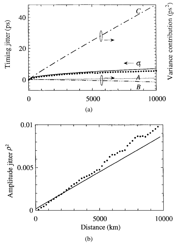
Fig. 11. Results for the same system as in Fig. 7, but for a 0-1-1-1-0 NRZ pulse.
