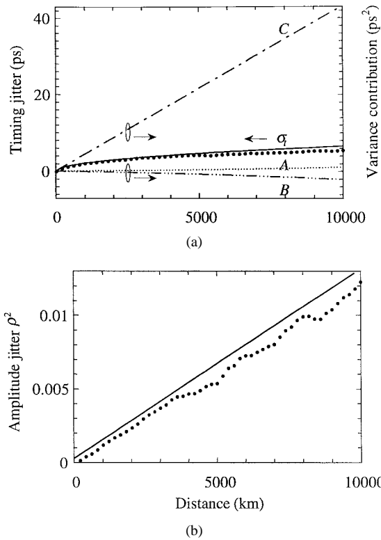
Fig. 9. Results for the same system as in Fig. 7, but for a 0-1-1-0 NRZ pulse.
