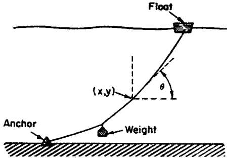
FIG. 1. —Mooring line.
