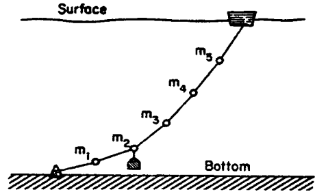
FIG. 2. —Discrete representation.
