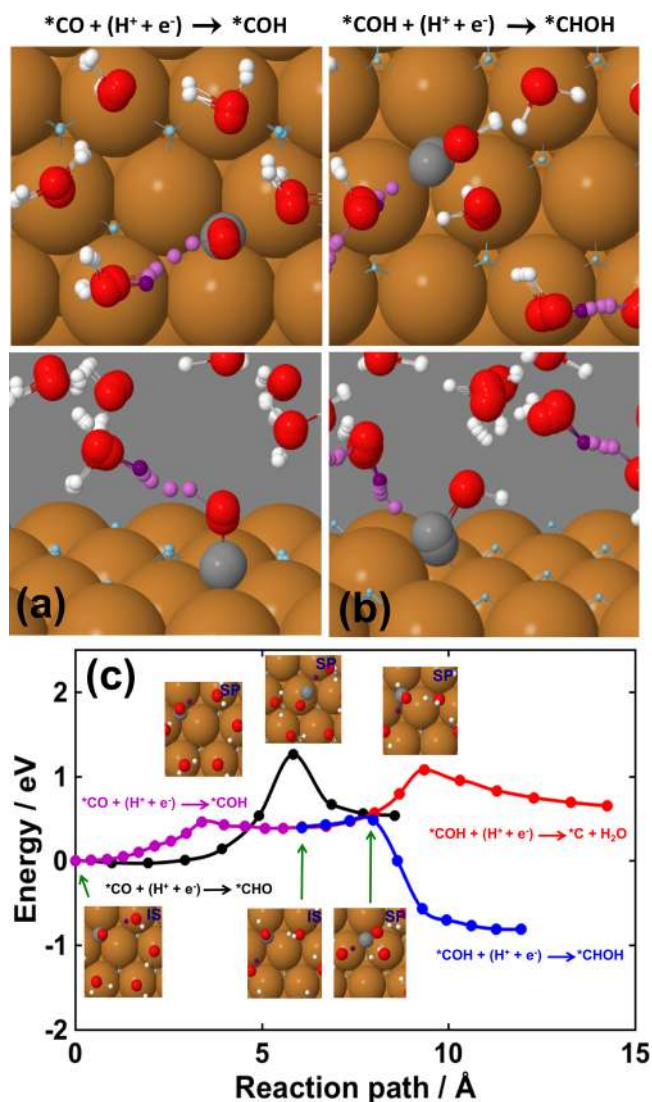
Figure 1. Minimum energy paths for two steps in the optimal CO 2 RR mechanism at a Cu(111) electrode. (a) and (b): Five positions of the transferred proton (purple, with a darker color representing the initial state), the H atoms (blue for adatoms, white in H 2 O molecules), O atoms (red), and C atoms (gray) starting with the initial state and ending at the saddle point on the energy surface. Only the initial configuration of the Cu atoms is shown for clarity. (c) Energy along the minimum energy paths for elementary proton–electron transfer steps where the initial state corresponds to -0.9 V potential. First, reduction of *CO to *COH (purple curve) and to *CHO (black curve). Second, *COH is further reduced to form *CHOH (blue curve) or *C and H 2 O (red curve). The calculations shown here are for a finite system where the applied potential changes along the path. The activation energy obtained from an extrapolation to an infinite system is given in Figure 2.
