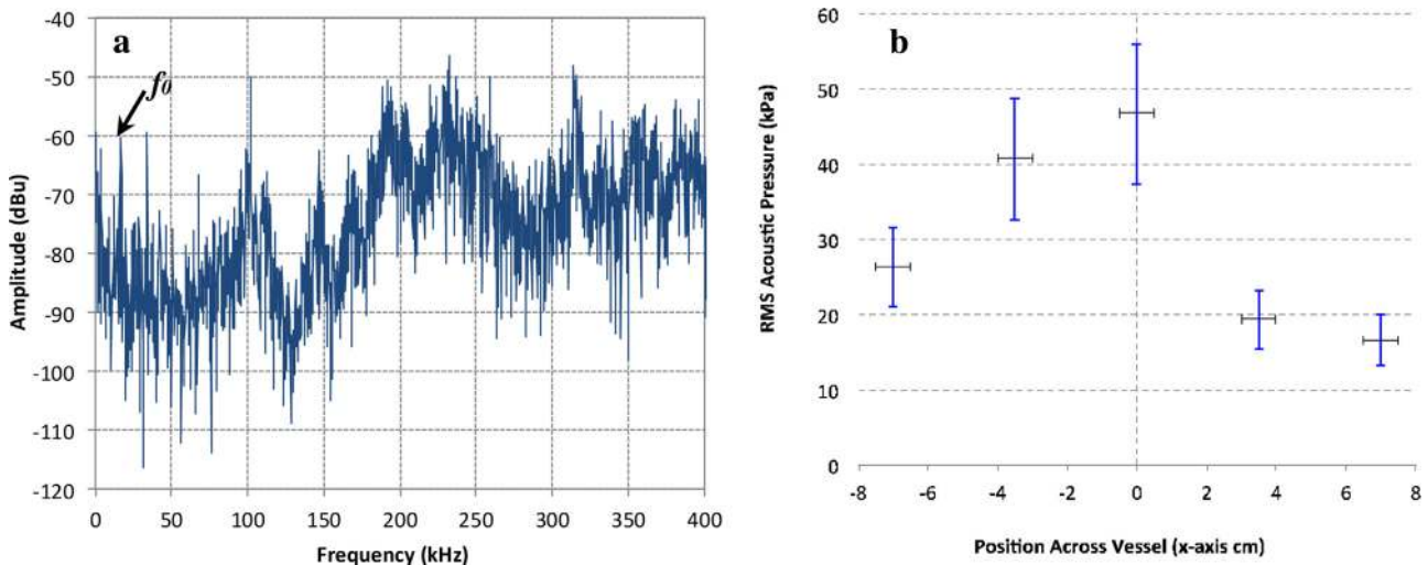
Fig. 16. (a) Typical example of acoustic spectrum generated by the magnetostrictive ultrasonic transducer at 17.5 kHz driving frequency and measured with the cavitometer tip positioned about 3–4 cm below the sonotrode's tip surface. (b) Variation in RMS acoustic pressure of the driving frequency with x-axis position across the cylindrical vessel.
