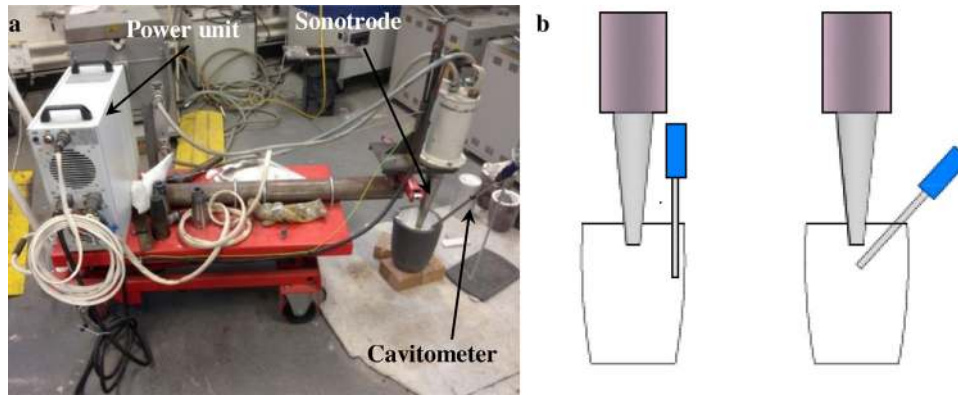
Fig. 15. (a) Experimental test rig for molten Al (b) a scheme showing positions of the cavitometer: near the side wall at 7 cm from the sonotrode and directly under the sonotrode at an angle of 35° (measurements were also performed at half-radius, not shown here).
