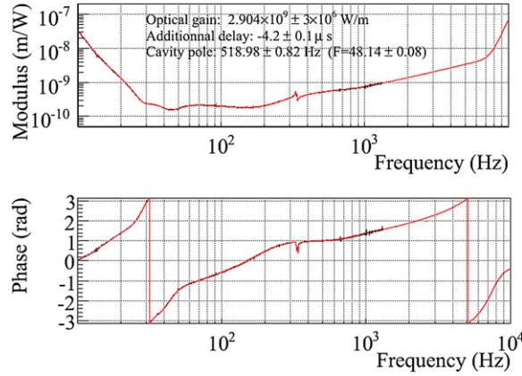
Figure 19. Virgo TF: modulus and phase in the range 10 Hz to 10 kHz (29 December 2009). The data are in black (only the points with coherence higher than 70% are shown). The continuous red line is the Virgo TF model: it is a copy of the measurements below 900 Hz, and is then extrapolated at higher frequency.
