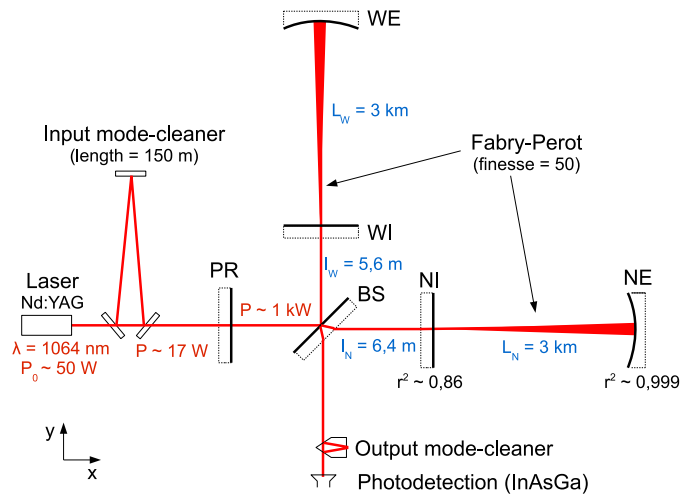
Figure 1. Optical scheme of Virgo.
