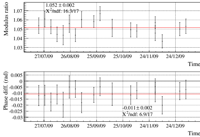
Figure 12. Stability of the LN to HP ratio (WE mirror, coil up) during VSR2, shown at 117 Hz. The average modulus and phase values are given and shown as the red line. The \chi^2/ndf assuming a constant response is given.
