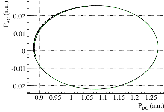
Figure 4. Example of the ac versus dc signals in a free swinging Michelson configuration (asymmetric Michelson) along with the fitted ellipse (green curve).
