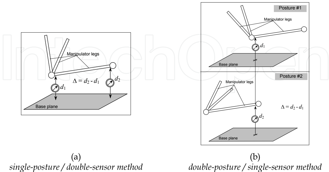
Fig. 4. Measuring the leg parallelism with respect to the base plane
