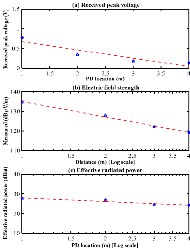
Figure 15. (a) Peak voltage, (b) Electric field strength, and (c) ERP as function of antenna distance from the floating electrode PD emulator.
