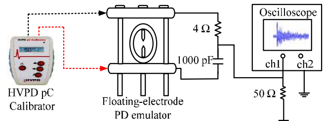
Figure 13. Measurement circuit for emulator calibration.
