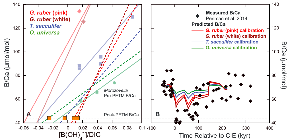
Figure 1. Modern B/Ca proxy calibrations are not applicable to the PETM B/Ca excursion. (a) Calibrations for B/Ca versus pH in G. ruber (white [Henehan et al., 2015] and pink [Allen et al., 2012]), T. sacculifer [Allen et al., 2012], and O. universa [Allen et al., 2011] are shown (solid colored lines and symbols). The horizontal dashed black lines indicate average pre-PETM and peak-PETM B/Ca ratios from the M. velascoensis study of Penman et al. [2014] (black diamonds). When the calibrations of T. sacculifer and O. universa are shifted through the pre-PETM B/Ca average (dotted lines), negative seawater [B(OH) 4 - ]/DIC ratios are predicted at the peak-PETM (orange squares). (b) The predicted B/Ca shift resulting from the ~0.3 unit pH decline estimated from boron isotope measurements across the PETM [Penman et al., 2014]. The colored lines show the proportion of the B/Ca excursion that each calibration can explain.
