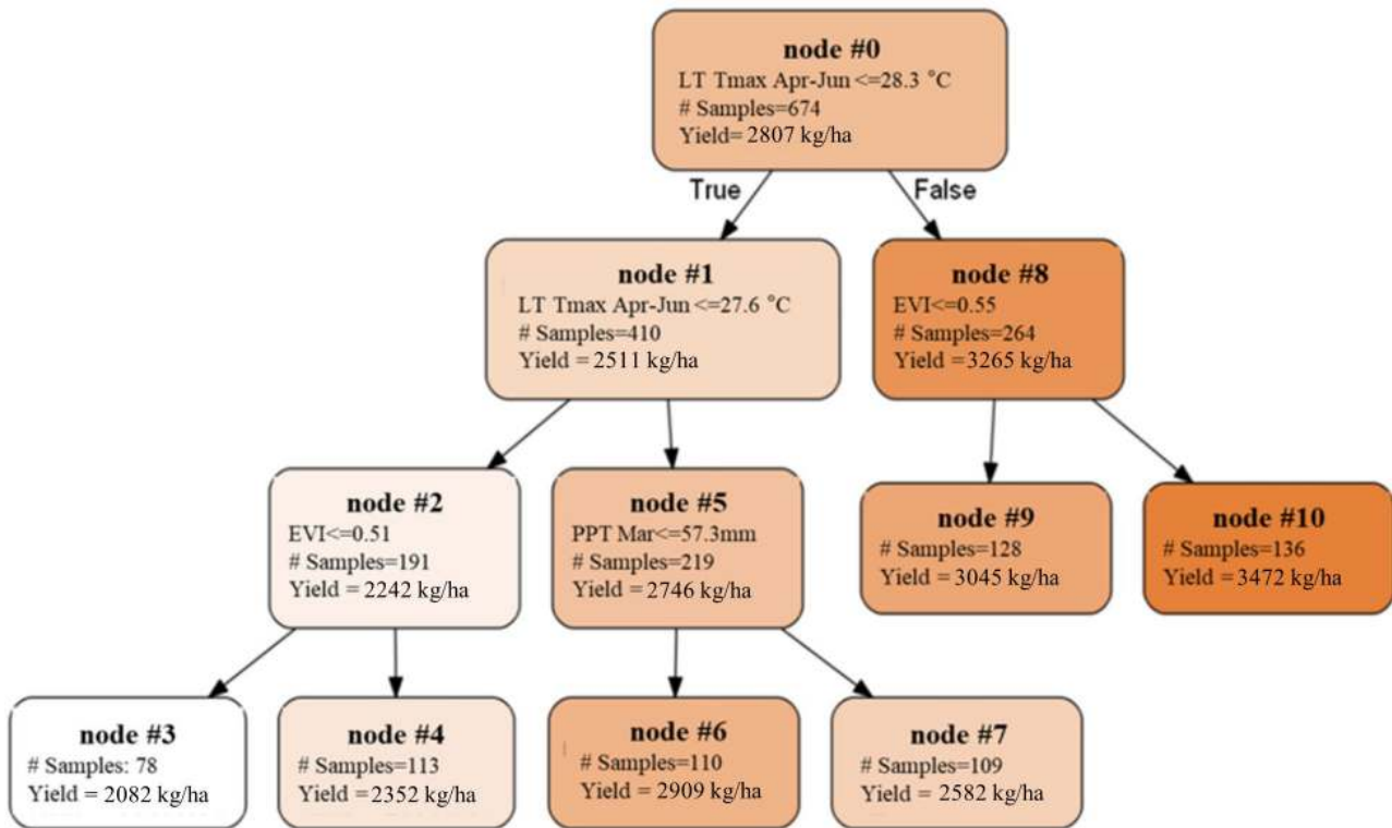
FIGURE 10 | Single decision tree built upon mature orchards using five important variables as predictors. Nodes with higher yields were represented with darker colors.
