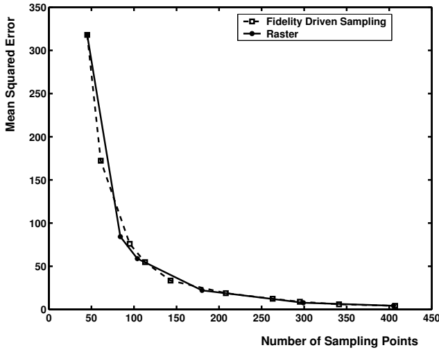
Figure 11: Mean Squared Error for reconstructions of the environmental field of Figure 8 as a function of sampling points comparing Fidelity Driven with raster sampling. Note that while raster sampling may exhibit a large variation in error with choice of sample density, Fidelity Driven sampling autonomously seeks a low value.
