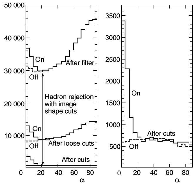
FIG. 44. Suppression of hadronic background through image shape analysis of the extragalactic Markarian 501 point source, observed by the HEGRA telescope. The right figure shows on an expanded scale the \gamma /hadron ratio after optimized cuts, with the \gamma signal concentrated at values \alpha < 10^\circ . “ON” (“OFF”) refers to ON (OFF) -source data (Barrio et al. , 1998).
