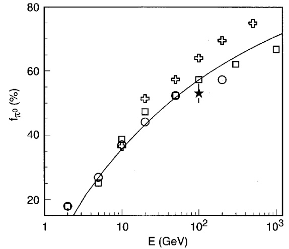
FIG. 27. The fraction of \pi^0 s, f(\pi^0) , produced in hadronic showers versus energy. The star is a measurement, squares are GCALE, circles GEISHA, and crosses CALOR predictions. One parametrization is also shown. From Kulchitsky (2000).
