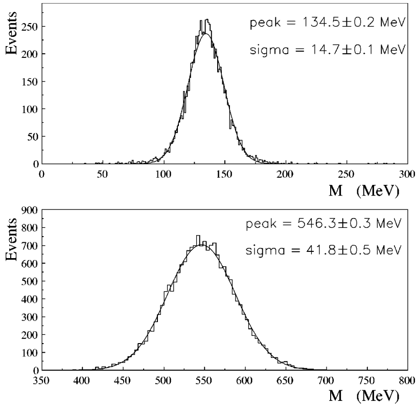
FIG. 14. Invariant mass distributions of photon pairs from \phi \rightarrow \pi^+ \pi^- \pi^0 events with \pi^0 \rightarrow \gamma\gamma (top) and from \phi \rightarrow \eta\gamma events with \eta \rightarrow \gamma\gamma (bottom), as reconstructed in the KLOE calorimeter (Antonelli et al. , 1995; Adinolfi et al. , 2002).
