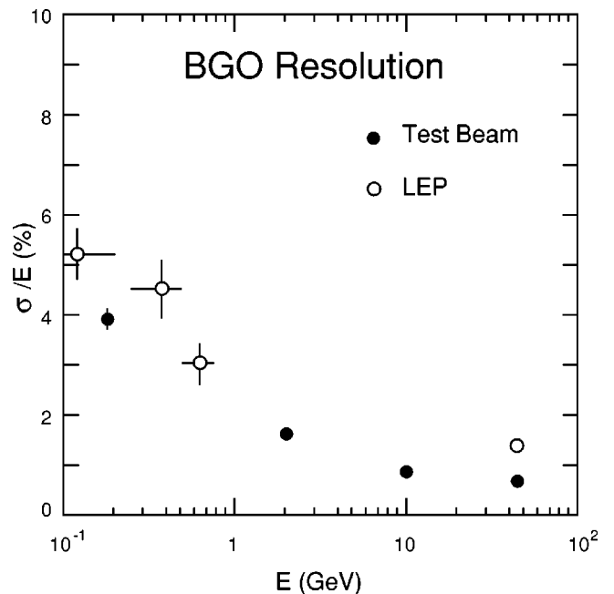
FIG. 7. Energy resolution of the L3 electromagnetic calorimeter as a function of energy, as obtained with test beam electrons (closed circles) and with physics data at LEP (open circles). From Karyotakis (1995).
