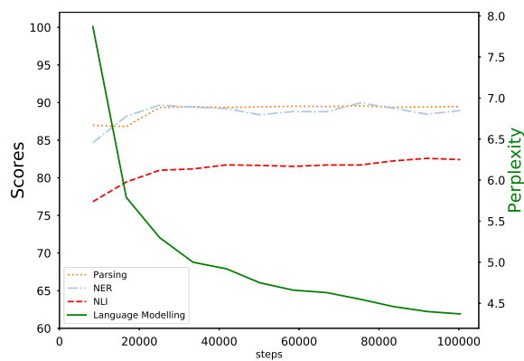
Figure 1: Impact of number of pretraining steps on downstream performance for CamemBERT.
