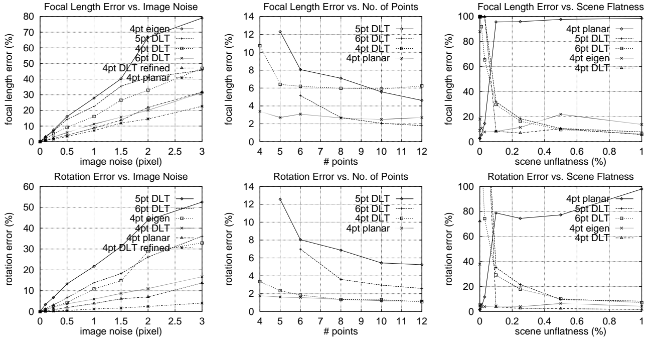
Figure 1: Left: Focal length & rotation error vs. noise, for each method’s minimal point number and preferred scene fitness. Middle: Error vs. number of points for 0.5 pixels noise. Right: Error vs. scene fitness for minimal point numbers.
