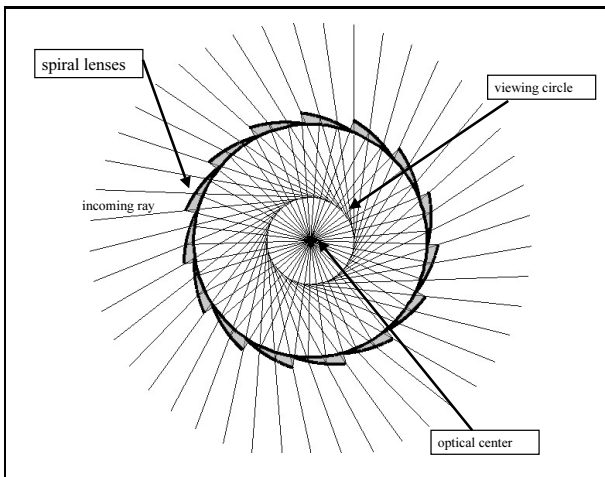
Figure 11. A collection of identical short spiral lens positioned on a circle. A Fresnel-like lens can be built with thousands of lens segments. Capturing the panorama can be done by an Omni Camera at the center of the viewing circle.
