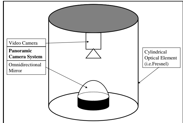
Figure 12. An omnidirectional camera at the center of the viewing circle enables the creation of a full 360 degrees left-image or a right-image.
