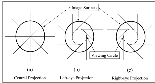
Figure 2. Circular projections. The projection from the scene to the image surface is done along the rays tangent to the viewing circle. (a) Projection lines perpendicular to the circular imaging surface create the traditional single-viewpoint panoramic image. (b-c) Families of projection lines tangent to the inner viewing circle form the multiple-viewpoint circular projections.
