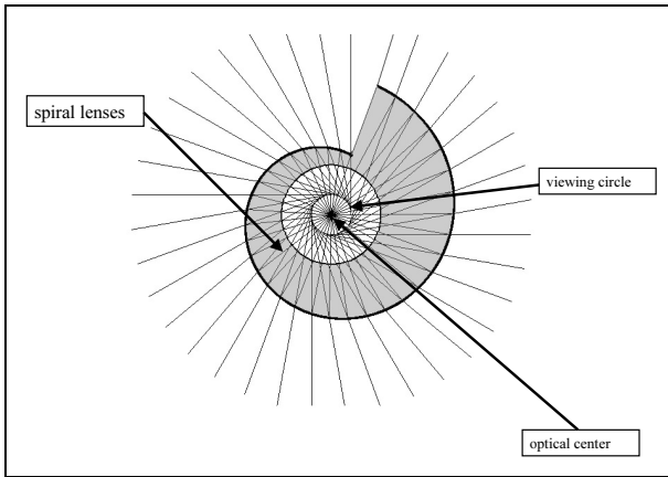
Figure 10. A spiral shaped lens. The diacaustic of the lens' outer curve is a circle (the viewing circle). Capturing the panorama can be done by an omnidirectional camera at the center of the viewing circle.
