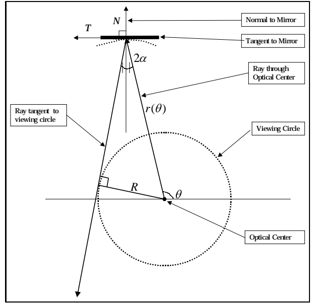
Figure 6. Differential conditions at a mirror patch: The optical center is at the center of the viewing circle of radius R , and the mirror is defined by its distance r(\theta) from the optical center. A ray passing through the optical center hits the mirror at an angle \alpha to the normal, and is reflected to be tangent to the viewing circle.
