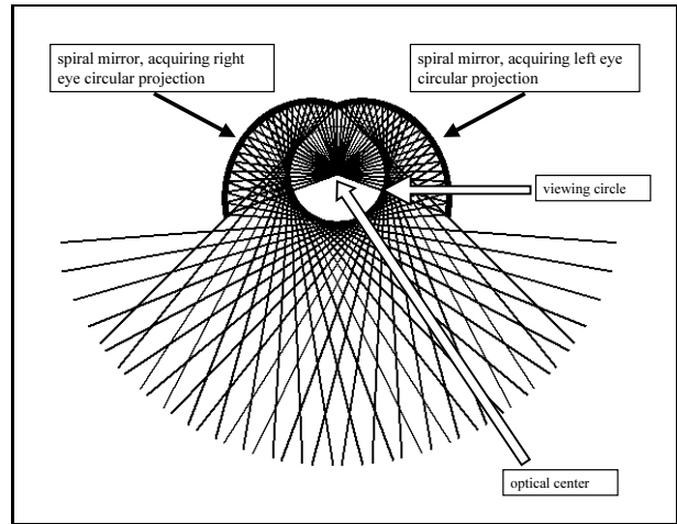
Figure 9. Two spiral shaped mirrors sharing the same optical center and the viewing circle. One mirror for the left-circular-projection and one for the right-circular-projection.
