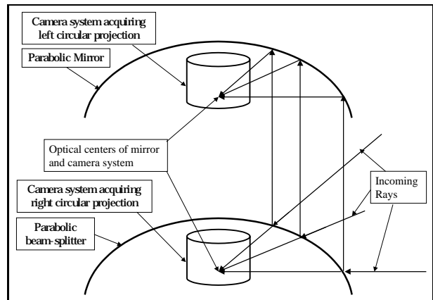
Figure 13. A setup for simultaneous capture of both left and right panoramas. A beam splitter is used to split the rays between two lens system. The horizontal rays enter into the bottom lens system for the right eye. The upward rays are reflected by a mirror into the upper lens system for the left eye.
