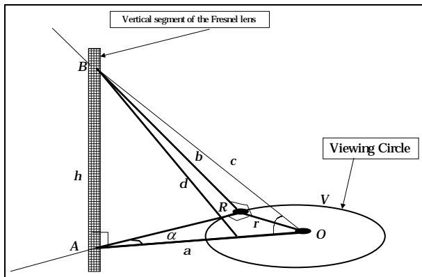
Figure 14. Vertical deflection of rays is necessary in order to assure that every viewing direction will have a single viewpoint on the viewing circle.
