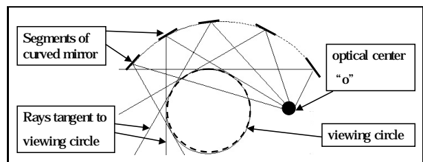
Figure 5. The spiral mirror: All rays passing through the optical center o will be reflected by the mirror to be tangent to the viewing circle V . This implies that rays tangent to the viewing circle will be reflected to pass through the optical center.
