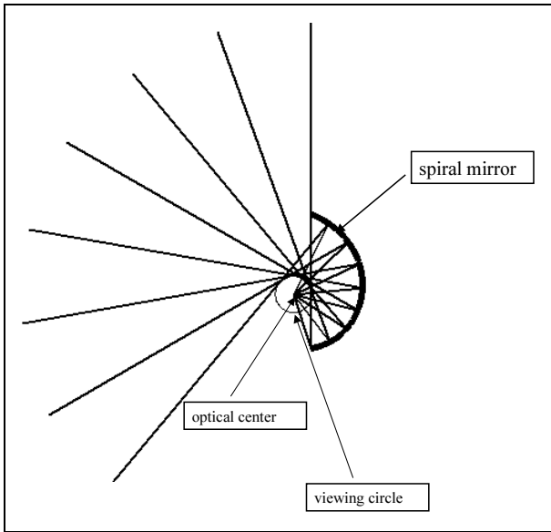
Figure 8. A spiral mirror where the optical center is at the center of the viewing circle.
