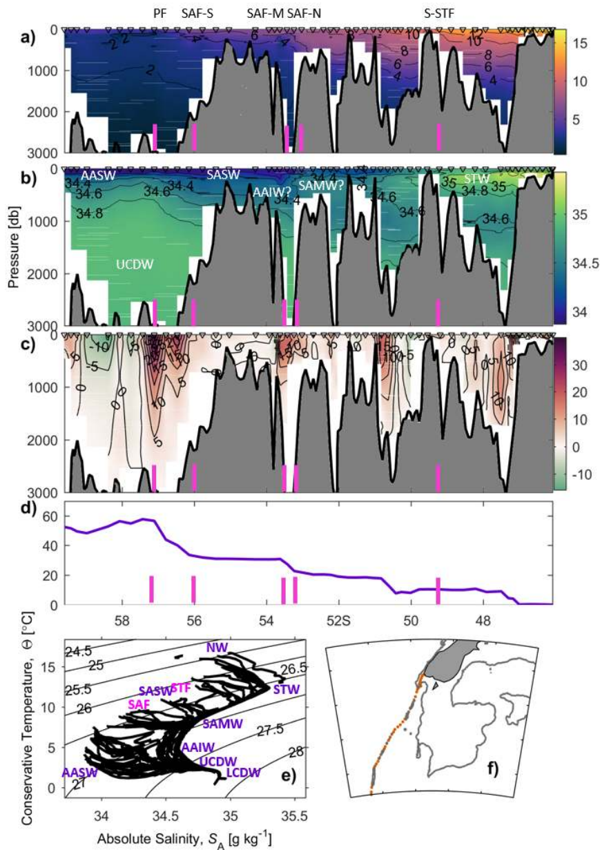
Figure 3. Macquarie Ridge: a) conservative temperature, contours every 2^\circ\text{C} , b) absolute salinity, contours every 0.2 \text{ g kg}^{-1} , c) geostrophic velocity, contours every 5 \text{ cm s}^{-1} positive values to the east, d) cumulative transport ( S_v ), e) \Theta - S_A diagram and f) transect position. Positions of the stations are marked on the top of the figure, fronts are marked with a magenta bar. Bathymetric features indicated on Fig. 1.
