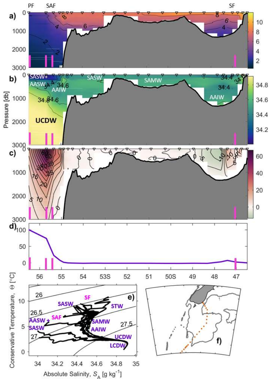
Figure 5. Western Campbell Plateau: a) conservative temperature, contours every 2^\circ C , b) absolute salinity, contours every 0.2\ g\ kg^{-1} , c) geostrophic velocity, contours every 5\ cm\ s^{-1} positive values to the east, d) cumulative transport (Sv), e) \Theta - S_A diagram and f) transect position. Positions of the stations are marked on the top of the figure, fronts are marked with a magenta bar. Bathymetric features indicated on Fig. 1. Note Southland Front (SF).
