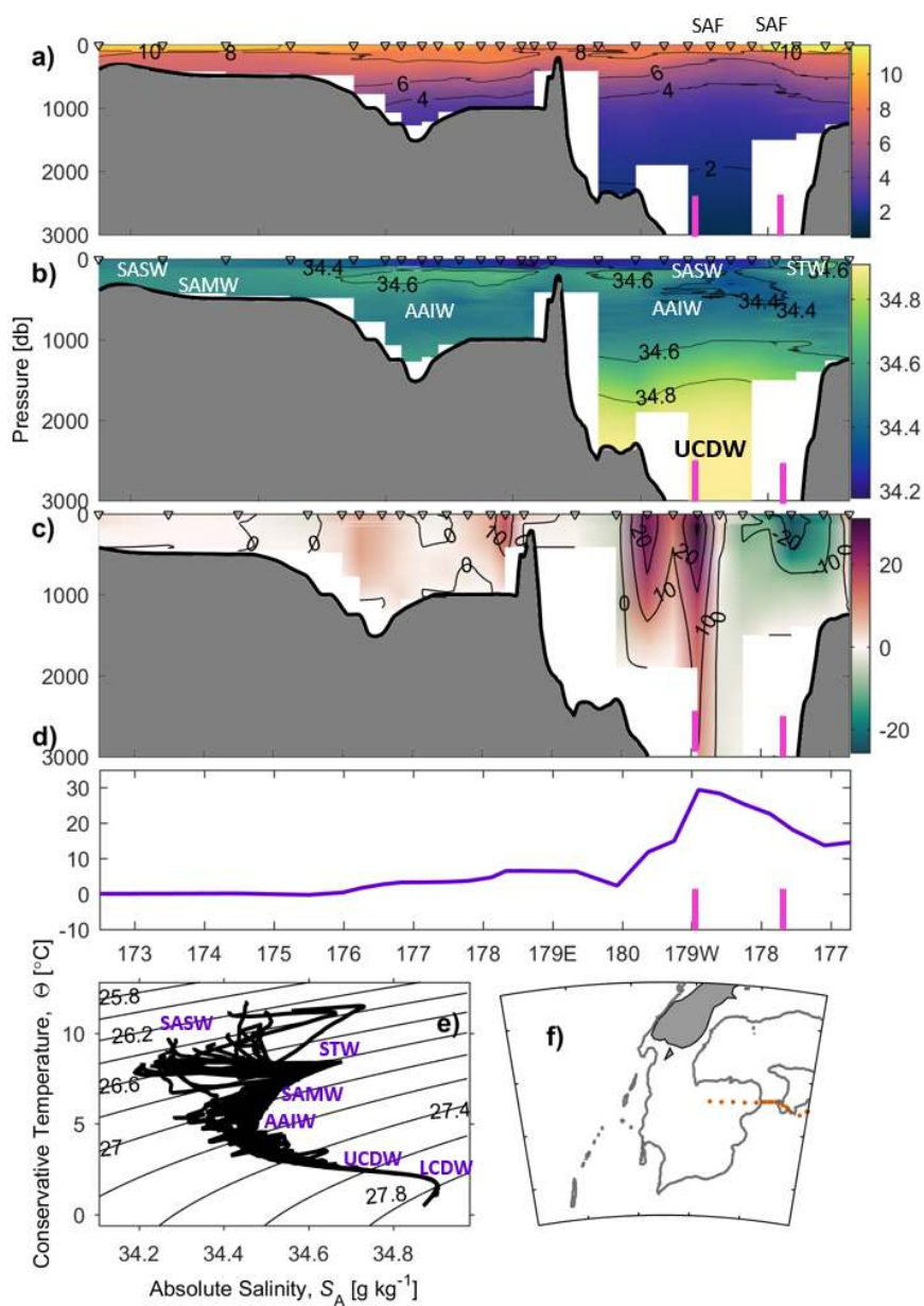
Figure 8. Pukaki Saddle: a) conservative temperature, contours every 2^{\circ}\text{C} , b) absolute salinity, contours every 0.2 \text{ g kg}^{-1} , c) geostrophic velocity, contours every 10 \text{ cm s}^{-1} positive values to the east, d) cumulative transport ( \text{Sv} ), e) \Theta - S_A diagram and f) transect position. Positions of the stations are marked on the top of the figure, fronts are marked with a magenta bar. Bathymetric features indicated on Fig. 1.
