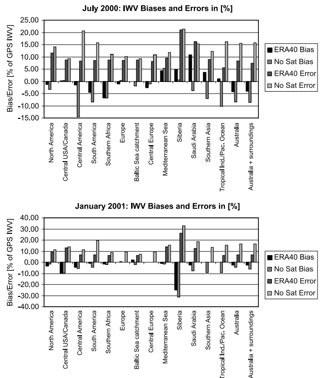
Figure 4. IWV bias and total error for (top) July 2000 and (bottom) January 2001 from comparison with GPS measurements in selected areas (see Table 4). Darker shaded vertical bars indicate the results from ERA40; lighter shaded bars indicate results from the NOSAT experiment. Note the dry bias, particularly in the NOSAT experiment.
