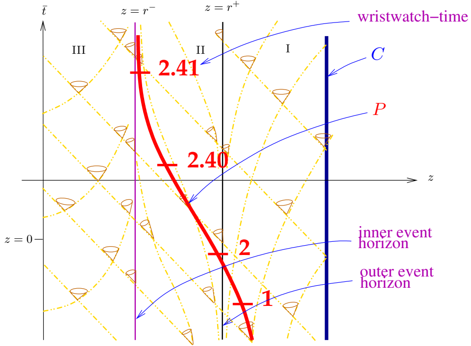
Fig. 9. The “ tz -slice” of spacetime of slowly rotating black hole in coordinates where z is the axis of rotation of black hole. The pattern of light cones between the two event horizons r^- and r^+ illustrates that P can decelerate so much in this region that he will receive outside of r^- all messages sent by C . r^+ is the outer event horizon, r^- is the inner event horizon, z = 0 is the “center” of the black hole as in Figure 8. The tilting of the light cones indicates that not even light can escape through these horizons. That there is an outward push counteracting gravity can be seen by the shape of the light-cones in region III (central region of the black hole). The time measured by P is finite (measured between the beginning of the experiment and the event when P meets the inner event horizon at b ) while the time measured by C is infinite.
