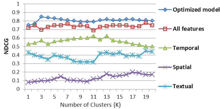
Fig. 6. Comparison of different models for the event identification task according to NDCG scores
