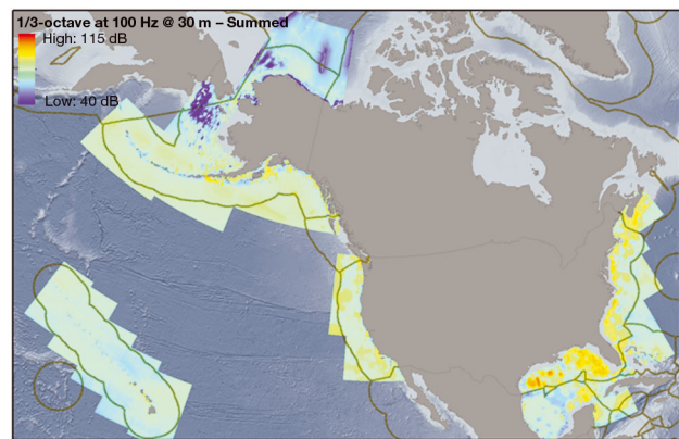
Fig. 2. Predicted low-frequency (one-third octave centered at 100 Hz) average annual noise levels (equivalent, unweighted sound pressure level in decibels re 1 µPa) at 30 m depth, summing contributions from a variety of human activities (see http://cetsound.noaa.gov/sound_data ) within the US Exclusive Economic Zone (brown lines)
