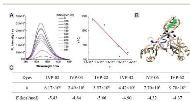
Fig. 9 (A) Fluorescence titration (left) of IVP-02 with RNA and the fitted curve (right) according to the Scatchard equation. (B) The binding mode of IVP-02 to RNA. (C) Binding constant ( k ) and binding energy ( E ) of IVP molecules to RNA.
