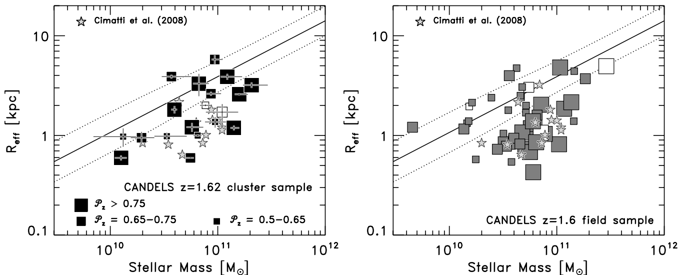
Figure 4. Left panel shows the relation between the circularized effective radii and stellar mass for quiescent galaxies in the z = 1.62 cluster for galaxies with projected distances R_{\text{proj}} < 1.5 Mpc from the cluster center and \mathcal{P}_z > 0.5 . The right panel shows the same relation for z = 1.6 quiescent galaxies in the field, selected in the same way as the cluster galaxies but with R_{\text{proj}} > 3 Mpc. In both panels, the size of the data point (boxes) scales with \mathcal{P}_z , as indicated in the legend of the left panel. The unfilled boxes denote objects detected at 24 \mu\text{m} with f_\nu(24 \mu\text{m}) \geq 50 \mu\text{Jy} . The filled stars correspond to the 1 < z < 2 early-type galaxy sample from Cimatti et al. (2008). Quiescent galaxies in the field at z \sim 1.6 in the CANDELS data have sizes similar to these other studies. There is a relative lack of compact quiescent galaxies in the cluster compared to galaxies in the field.
