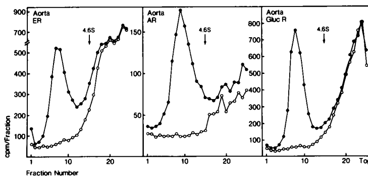
FIGURE 1 ER, AR, and GLUC R in dog aorta. Aortas were excised from three different dogs and cytosols were prepared and incubated 4 h at 0^{\circ}\text{C} with hormones. ER: 4 nM [ ^3\text{H} ]estradiol only ( \bullet ) or together with 400 nM diethylstilbestrol ( \circ ); cytosol from spayed female; 5.1 mg/ml protein. AR: 20 nM [ ^3\text{H} ]R1881 and 200 nM triamcinolone acetone only ( \bullet ) or with 2,000 nM R1881 added ( \circ ); cytosol from female; 10.6 mg/ml protein. GLUC R: 50 nM [ ^3\text{H} ]dexamethasone only ( \bullet ) or with 5,000 nM dexamethasone added ( \circ ); cytosol from female; 12.4 mg/ml protein. After charcoal treatment, aliquots of cytosol were layered over 5–20% sucrose density gradients and centrifuged in swinging bucket (ER, AR) or gradient reorienting rotors (GLUC R). Fractions were collected and counted. Sedimentation of ^{14}\text{C} -BSA is shown by arrows. ER: 207 fmol/mg DNA; AR: 153 fmol/mg DNA; GLUC R: 868 fmol/mg DNA.
