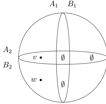
Figure 3: The corner diagram of (A_1, B_1) and (A_2, B_2) . By nestedness the bottom right corner and its two adjacent links are empty. The vertex w exists as (A_2, B_2) is proper. The vertex v exists as the connected set A_1 \setminus B_1 is not a subset of B_2 .
