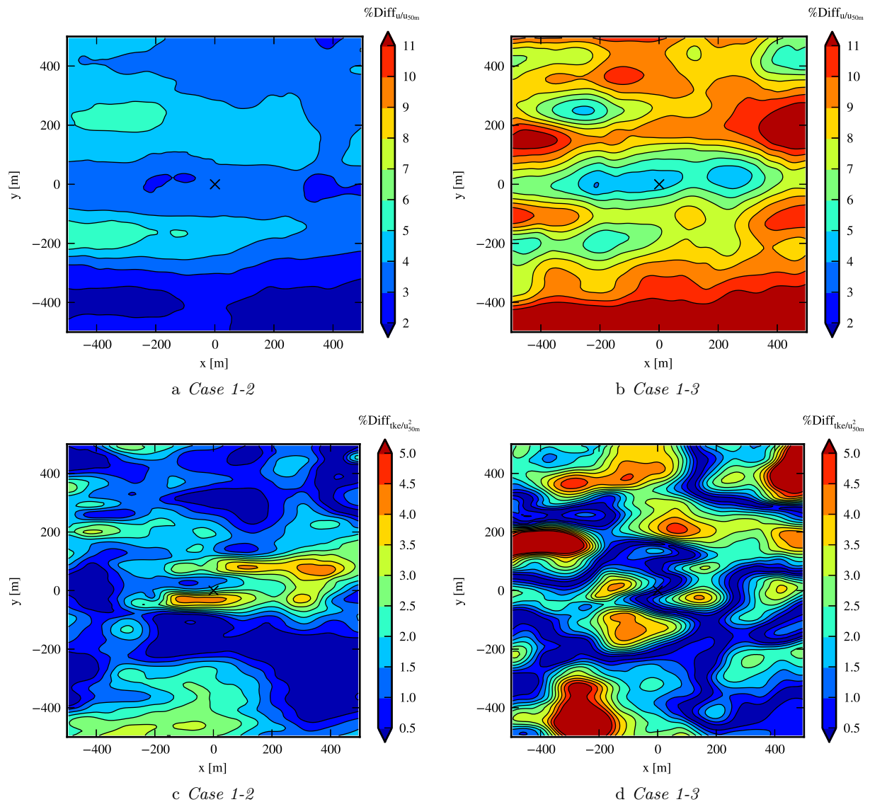
Figure 5. Percentage difference in u/u_{50m} and tke/u_{50m}^2 between Case 1 and Case 2 and Case 1 and Case 3 at 50 m above the ground level. The upstream farfield velocity u_{50m} at 50 m was used to normalize the fields. The flow direction goes from left to right.
