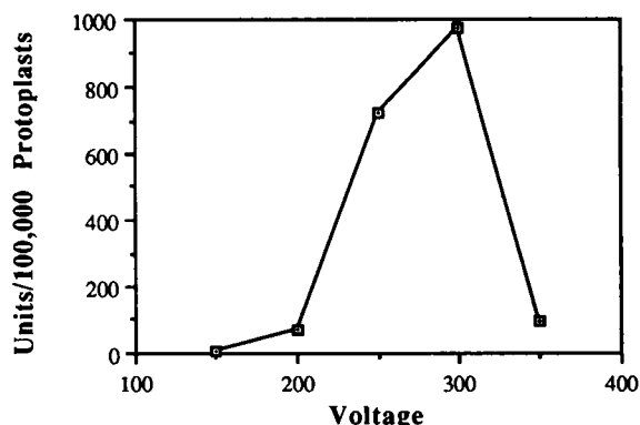
FIG. 2. Effect of voltage during electroporation of tobacco protoplasts with pRTL-GUS DNA. Equal numbers of protoplasts ( 4 \times 10^5 ) were electroporated at 150, 200, 250, 300, or 350 V (five pulses of 1-ms duration each). Lysates were prepared after an incubation of 15 h and assayed for GUS activity.
