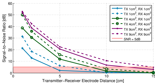
Figure 7. Ground-Coupling by Touch: The Signal-To-Noise Ratio with different receiver/transmitter distances and electrode sizes. The 5 dB SNR threshold results in a bit error rate (BER) of more than 20%, which means that many messages are corrupted.
