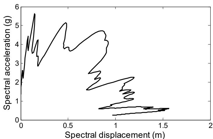
Figure 18. Example of a 5% damped elastic response spectrum in ADRS format for an accelerometer matching the EC08 1D response spectrum.
