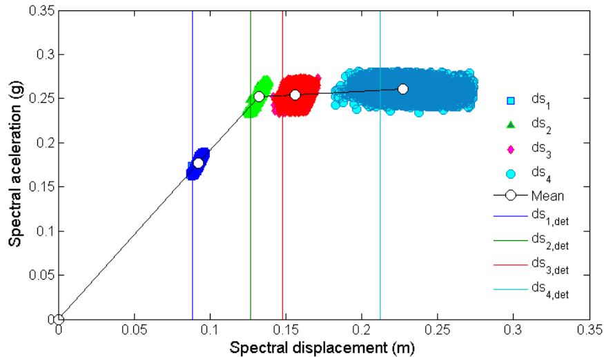
Figure 14. Damage states thresholds obtained with the probabilistic and deterministic approaches.
