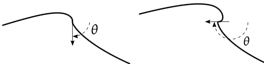
Figure 6: Topological wave state criteria. Left: breaking criterion with the interface presenting a vertical segment (-90 degrees angle). Right: overturning wave with the interface presenting both vertical and horizontal segments (-180 degrees angle).
