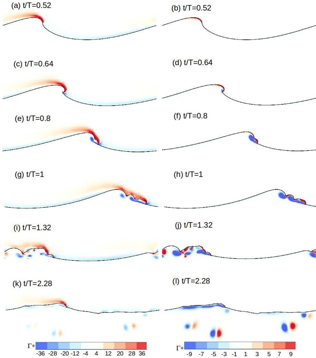
Figure 5: Evolution of a spilling-overturning breaker and its vorticity field \Gamma^* at different times, displayed both in the air and water (left) and only in the water (right) with a different color-scale. Initial conditions Re = 4 \times 10^4 , Bo = 70 , \epsilon = 0.45 . The wave begins to break (a-d) similar to figure 4 but with the interface almost overturning (c-d) and formation of bubbles after the breaking stage (i-j). The turbulent breakdown appears stronger and several vortices are generated in the water (k-l).
