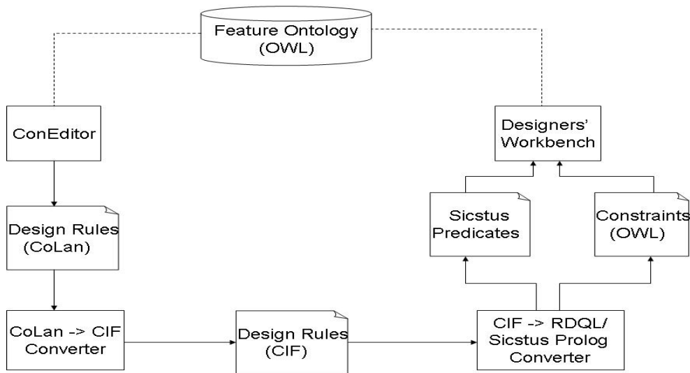
Figure 4.5: Framework of ConEditor and Designers' Workbench
