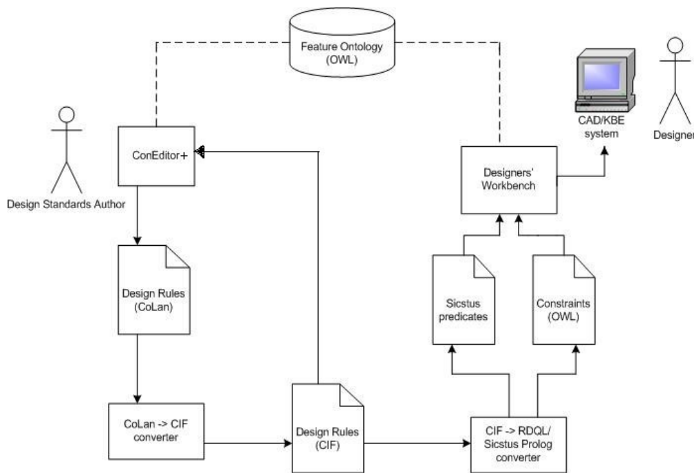
Figure 8.1: Proposed System Architecture
