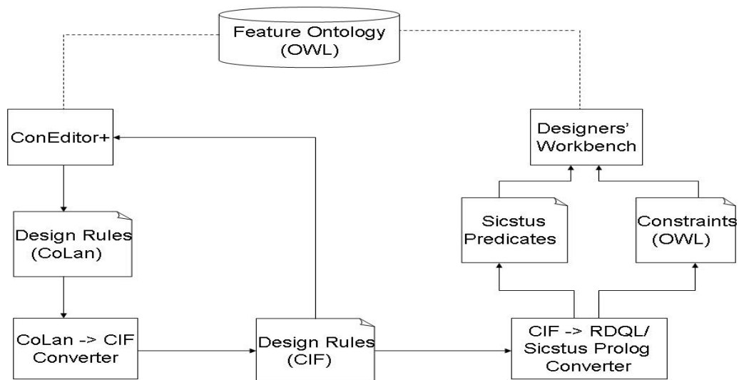
Figure 6.3: Framework of ConEditor+ and Designers' Workbench
