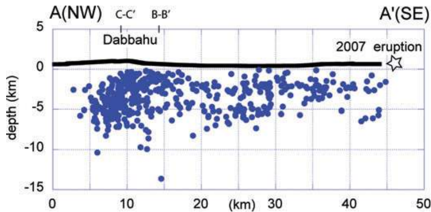
Figure 7. Seismicity within a \leq 4 km swath projected onto the line of Profile A-A shown in Fig. 4. Crossing points of Profiles B and C are indicated above the graph. The shallowest events correspond to surface breaks described in Rowland et al. (2007). Patterns in the Dabbahu complex are shown in more detail along- and across-axis profiles in Fig. 8.
