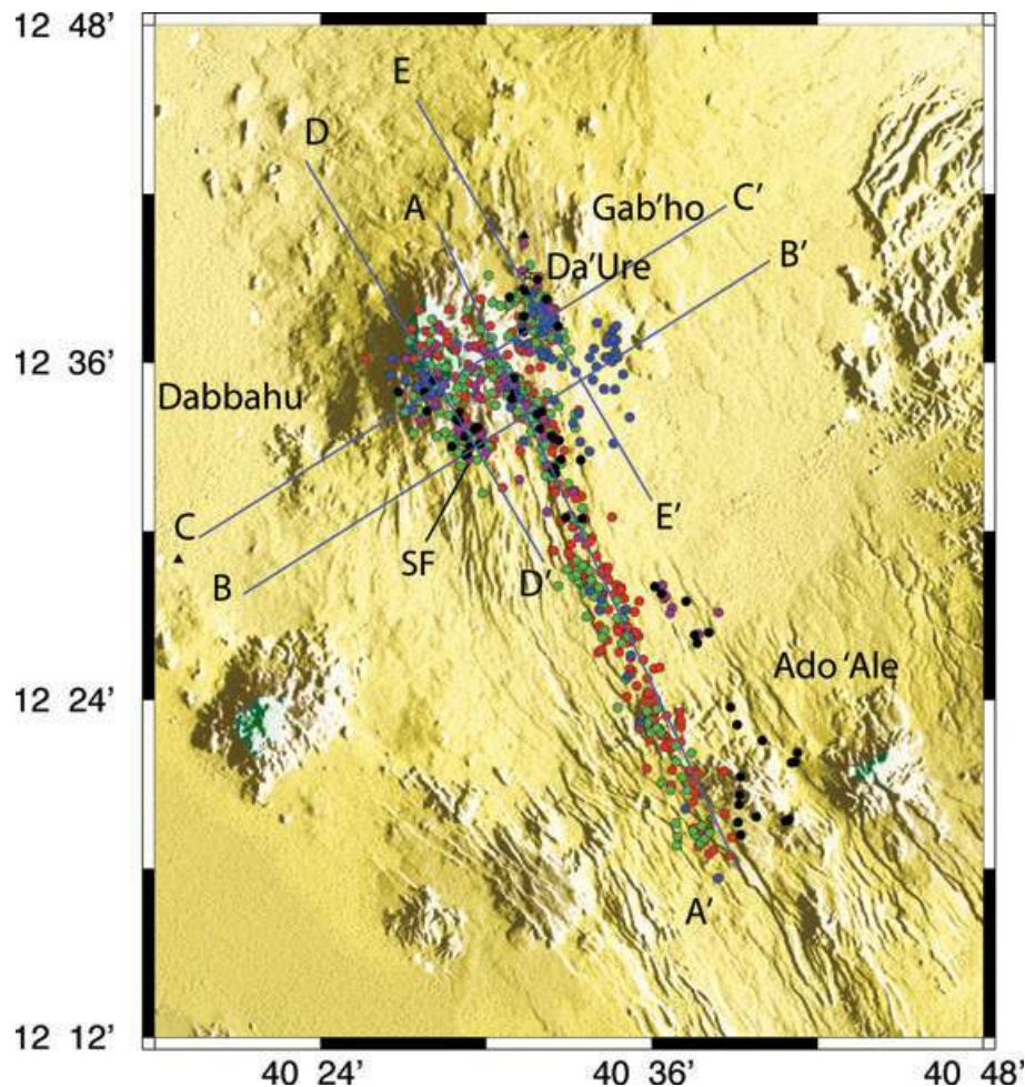
Figure 4. Earthquake epicentres relocated using the double difference method of Waldhauser & Ellsworth (2000). A-A , B-B , C-C , D-D E-E mark the locations of topography and seismicity profiles shown in Figs 7 and 8. Colours signify temporal variations: red, 2005 October 19–31; green, 2005 November 1–30; blue, 2005 December 1–31; violet, 2006 1–31; black, 2006 February 1–March 30. Ado 'Ale, Dabbahu, Gab'ho are silicic volcanoes.
