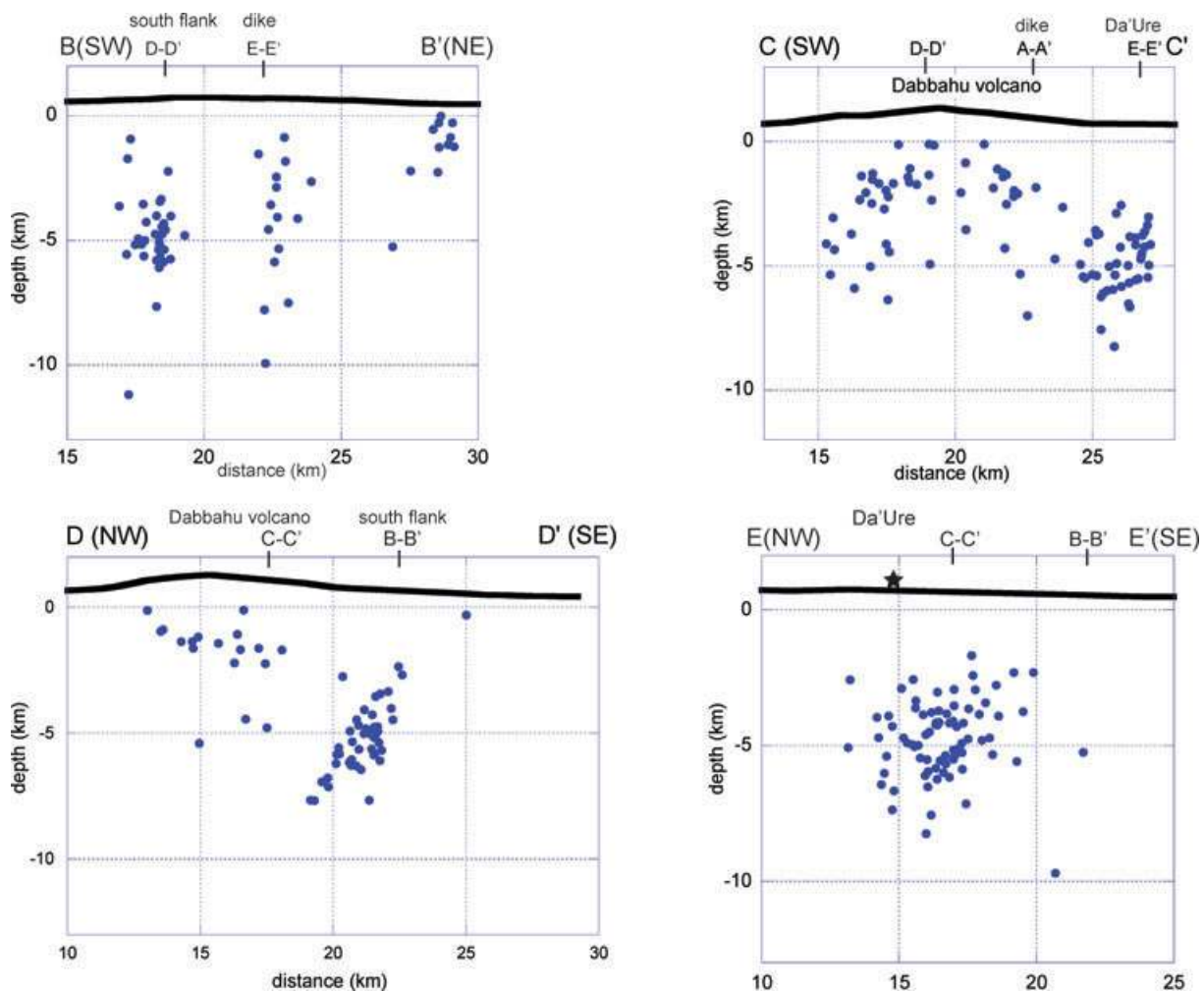
Figure 8. Seismicity in \leq 2 km-swaths projected on the line of profiles B-B, C-C, D-D, and E-E shown in Fig. 4. All profiles are shown at true scale to enable correlations with focal mechanisms and fault slip data. Crossing points of profiles are indicated above the profile (Figs 4 and 7).
