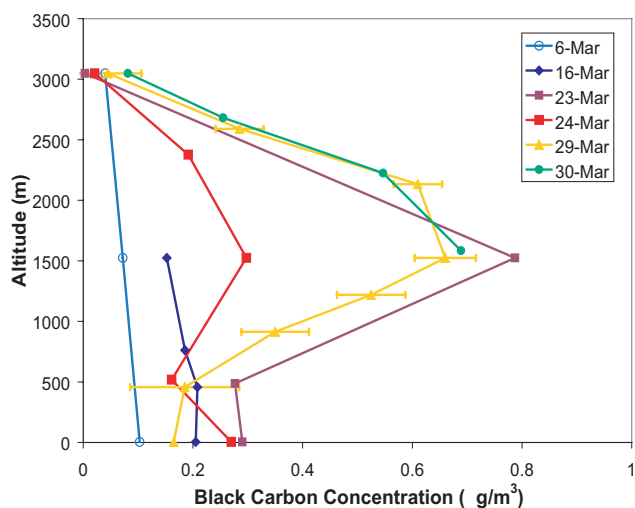
Fig. 13. Black carbon concentration altitude profiles during MAC experiment (March 2006). Error bars are only shown for a single flight to keep the plot legible and are representative of all flights.
