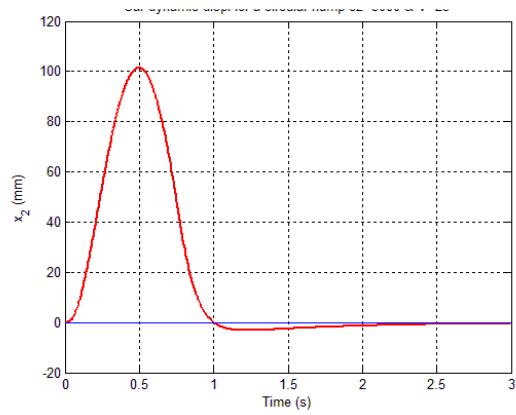
Fig.11 Sprung-mass displacement for c_2=5 kNs/m and V = 25 km/h.
