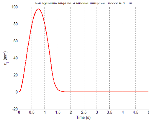
Fig.19 Sprung-mass displacement for c_2=15 kNs/m and V = 15 km/h.
