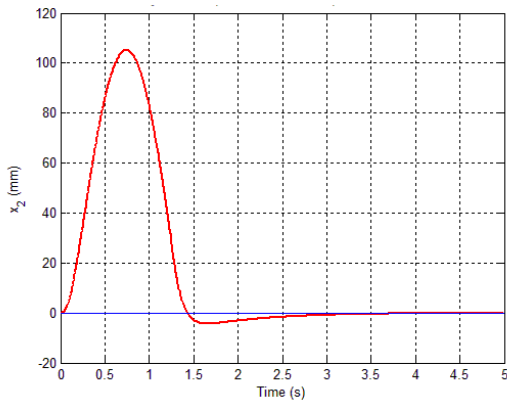
Fig.9 Sprung-mass displacement for c_2=5 kNs/m and V = 15 km/h.
