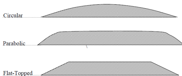
Fig.2 Three types of speed humps [22].
