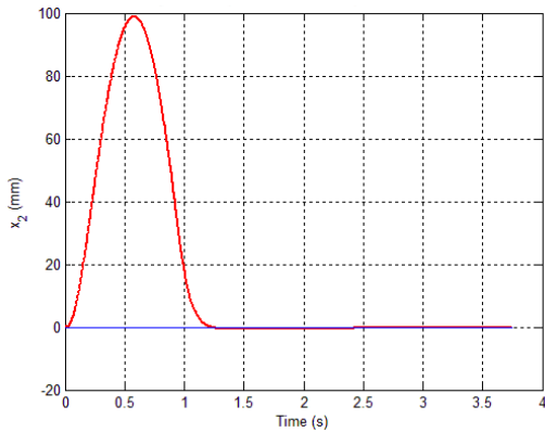
Fig.15 Sprung-mass displacement for c_2=10 kNs/m and V = 20 km/h.
