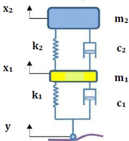
Fig.1 Quarter-car physical model [20].
