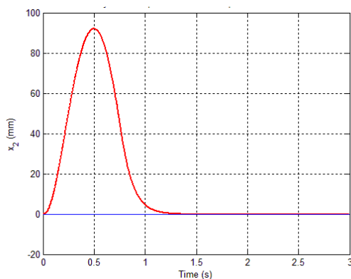
Fig.21 Sprung-mass displacement for c_2=15 kNs/m and V = 25 km/h.
