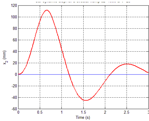
Fig.6 Sprung-mass displacement for c_2=1 kNs/m and V = 25 km/h.
