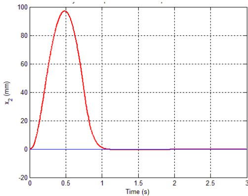
Fig.16 Sprung-mass displacement for c_2=10 kNs/m and V = 25 km/h.
