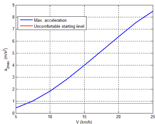
Fig.25 Maximum sprung-mass acceleration for c_2 = 15 kNs/m.
