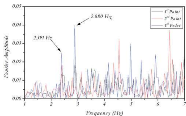
Figure 10 Fourier spectra in the X axis for the three points tested
