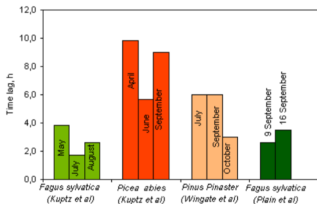
Fig. 2. Seasonal changes in time lag measured by tracing variations in \delta^{13}\text{C} at natural abundance level (Wingate et al., 2010; Kuptz et al., 2011a) or after ^{13}\text{C} pulse-labeling (Plain et al., 2009) in soil respiration and trunk respiration (at 1 m height; Kuptz et al., 2011a). Average values were calculated based on monthly ranges reported in Wingate et al. (2010).
