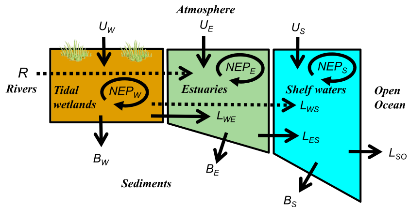
Figure 1. Conceptual diagram for the carbon balance of coastal ecosystems. The relevant fluxes are uptake of atmospheric CO 2 ( U ), burial of organic carbon ( B ), riverine input ( R ), and lateral transport ( L ). Subscripts W, E, S, and O represent tidal wetlands, estuaries, shelf waters, and the open ocean, respectively. Dashed arrows represent carbon pathways not directly passing through either tidal wetlands or estuaries. NEP = net ecosystem production.
