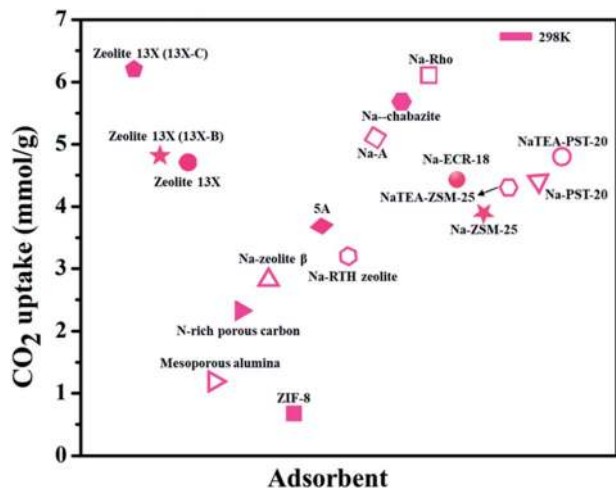
Fig. 9 \text{CO}_2 adsorption capacities of zeolite-based adsorbents (for some adsorbents \text{CO}_2 uptake units are converted from the originally reported ones).
