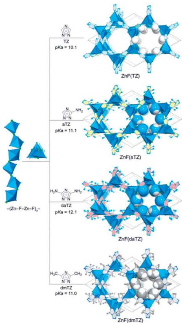
Fig. 5 Graphical illustration for the framework construction of a robust isorecticular metal triazololate (Reproduced with permission from ref. 51 Copyright© 2020, American Chemical Society).
