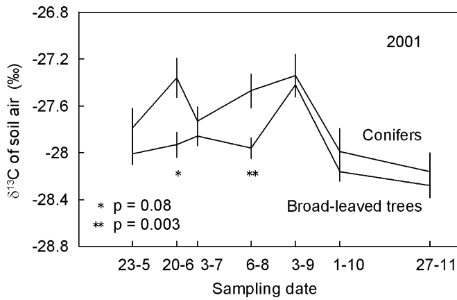
Fig. 4 Seasonal course of the \delta^{13}\text{C} values in soil air sampled near conifers and broad-leaved trees. During the whole growing season the \text{CO}_2 of soil air near conifers was less depleted in ^{13}\text{C} . Only data of the untreated area were used. Error bars indicate SE
