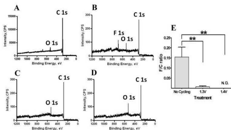
Figure 2. XPS spectra of PPF electrode surfaces. F 1s, O 1s and C 1s indicate characteristic peaks for fluorine, oxygen and carbon, respectively. (A) PPF electrode before any treatment. (B) PPF electrode after coating with silicon nitride, removal of insulation by etching with \text{CHF}_3/\text{O}_2 and subsequent immersion in buffer solution. (C, D) PPF electrode after 30 minute treatment with the 1.3 V waveform and the 1.4 V waveform, respectively. Each waveform was repeated at 60 Hz. (E) Summary of F/C atomic ratios for PPF electrodes before treatment and after 1.3 V, and 1.4 V treatments. N. D. – no fluorine was detected; double asterisk represents p < 0.01 for one way variance ANOVA statistical test ( n = 4 for each condition).
