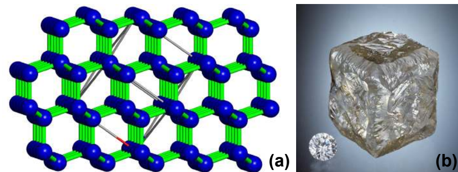
Figure 2. (a) The diamond (native C) crystal structure (cubic, space group Fd\bar{3}m ; a = 3.560 Å; Z = 8 ) features a framework of tetrahedrally coordinated carbon atoms. (b) A natural diamond crystal reflects the cubic crystal structure. The semi-translucent diamond cube (ref. no. S014632) is 24.3 \times 21.8 \times 21.7 mm in size and weighs 156.381 carats (31.3 gm) and is shown with a 1-carat diamond for scale. It is represented to be from Ghana. Photo courtesy of Harold and Erica Van Pelt. [Animation 2: For readers of the electronic version, click the image for an animation of the diamond crystal structure.]
