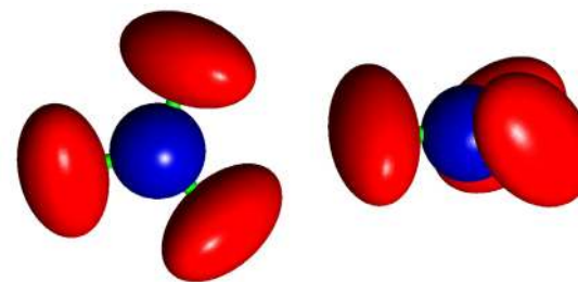
Figure 11. The rigid body librating \text{CO}_3^{2-} unit of the calcite and dolomite mineral groups. Blue and red ellipsoids represent carbon and oxygen atoms, respectively. [Animation 7: For readers of the electronic version, click the image for an animation with librating \text{CO}_3^{2-} .]
