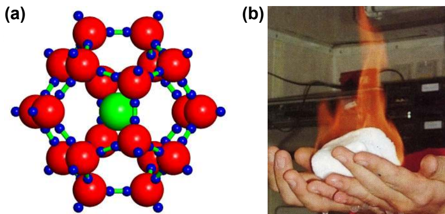
Figure 15. Methane hydrate. (a) The structure of methane hydrate [ \text{H}_2\text{O} \cdot \text{CH}_4 ] (cubic; space group Pm\bar{3}m ; a = 12 \text{ \AA} ). (b) Methane hydrate burns at room conditions, as the hydrate melts and methane is released. Photo courtesy of Jan Steffan, Expedition SO148, GEOMAR. [Animation 11: For readers of the electronic version, click the image for an animation of the methane hydrate crystal structure.]
