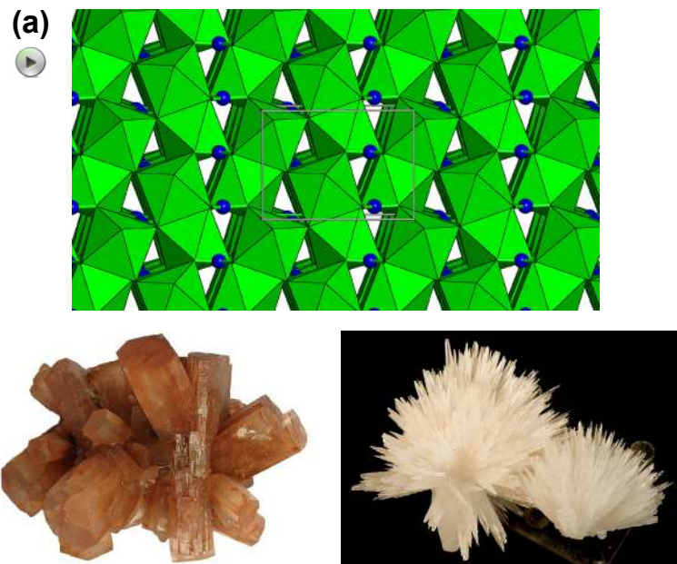
Figure 12. Aragonite Group. (a) The structure of aragonite ( \text{CaCO}_3 ) (orthorhombic; space group Pm\bar{c}n ; a = 4.960 \text{ \AA} ; b = 7.964 \text{ \AA} ; c = 5.738 \text{ \AA} ; Z = 4 ). Blue spheres are carbon atoms, whereas green polyhedral are \text{CaO}_9 groups. (b) The orthorhombic structure of aragonite is manifest in its common crystal forms, including tabular crystals from Tazouta Mine, Sefrou, Morocco (left) and acicular crystals from Transvall, South Africa. Photos courtesy of Rob Lavinski. [Animation 8: For readers of the electronic version, click the image for an animation of the aragonite crystal structure.]
