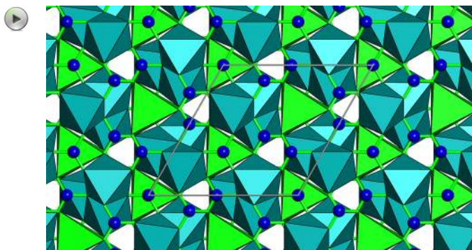
Figure 14. The structure of huntite [ \text{CaMg}_3(\text{CO}_3)_4 ]. (hexagonal; space group R\bar{3}2 ; a = 9.503 \text{ \AA} , c = 7.821 \text{ \AA} ; Z = 3 ). The huntite structure is unusual in the trigonal prism coordination of calcium, coupled with octahedral coordination of magnesium. [Animation 10: For readers of the electronic version, click the image for an animation of the huntite crystal structure.]
