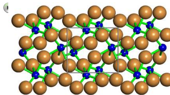
Figure 6. The structure of the iron carbide cohenite [(\text{Fe,Ni,Co})_3\text{C}] (orthorhombic, space group Pbnm ; a = 4.518 \text{ \AA} , b = 5.069 \text{ \AA} ; c = 6.736 \text{ \AA} ; Z = 4 ). Carbon and iron atoms appear in blue and gold, respectively. [Animation 4: For readers of the electronic version, click the image for an animation of the iron carbide cohenite crystal structure.]
