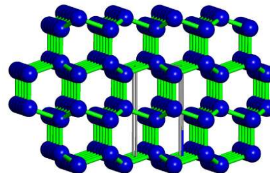
Figure 3. The lonsdaleite (native C) crystal structure (hexagonal, space group P6_3/mmc ; a = 2.52 Å; c = 4.12 Å; Z = 4 ). [Animation 3: For readers of the electronic version, click the image for an animation of the lonsdaleite crystal structure.]
