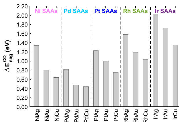
Fig. 5 The CO induced segregation energy \Delta E_{seg}^{CO} for a single dopant atom to migrate from the (111) surface into the “bulk” of group 11 metal host materials. Positive values indicate a preference for segregation of the dopant in the presence of CO to the surface, whereas negative values would indicate a preference for segregation into the bulk
