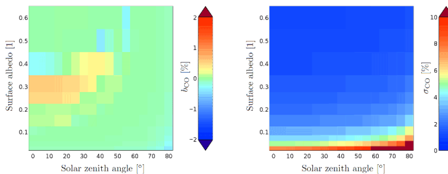
Figure 5. Retrieval bias b_{CO} (left panel) and retrieval noise \sigma_{CO} (right panel) for the clear sky conditions (without aerosol, clouds and cirrus) and for a viewing zenith angle (VZA) of 0^\circ as a function of solar zenith angle (SZA) and surface albedo A_s .
