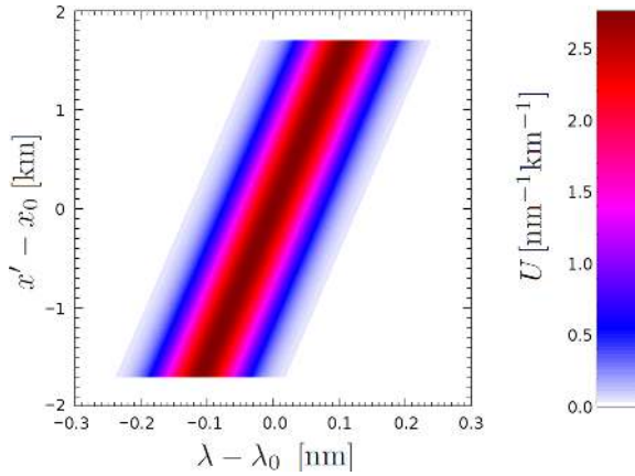
Figure B2. Instrument response function U(x_0, \lambda_0 | x, \lambda) as defined in Eqs. (B7) and (B8) with \Delta x = 3.4 km, \Delta w = 0.1 nm and b = 6.47 \times 10^{-2} \text{ nm km}^{-1} .
