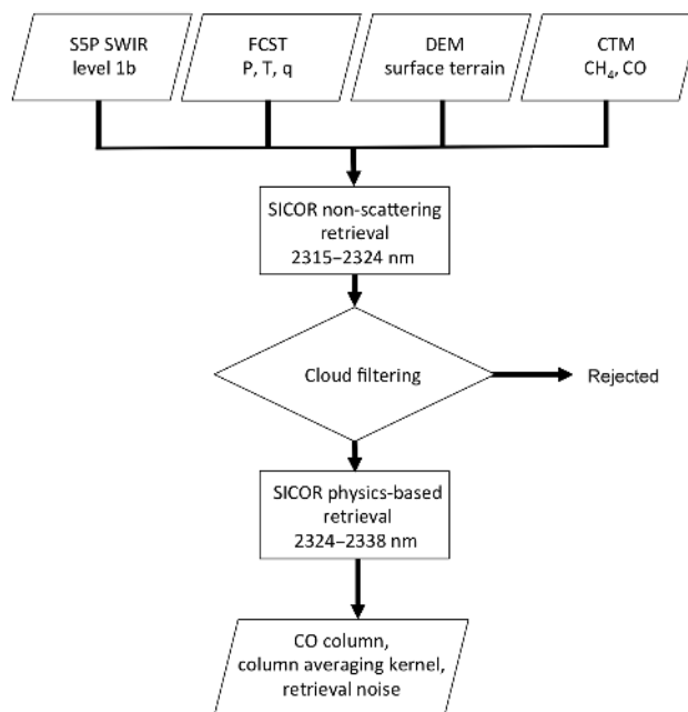
Figure 2. Flowchart of the SICOR algorithm.
