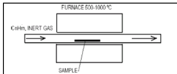
Figure 5: CVD reactor
