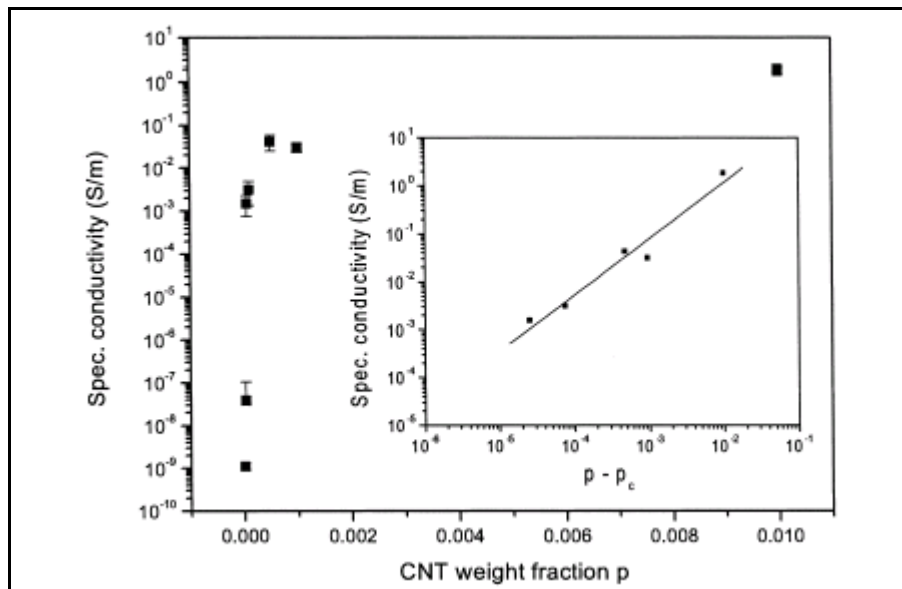
Figure 7: Semi-log plot 52 of the specific composite conductivity as a function of carbon nanotube weight fraction p : The insert shows a log-log plot of the conductivity as a function of p - p_c with an exponent t of 1.2
