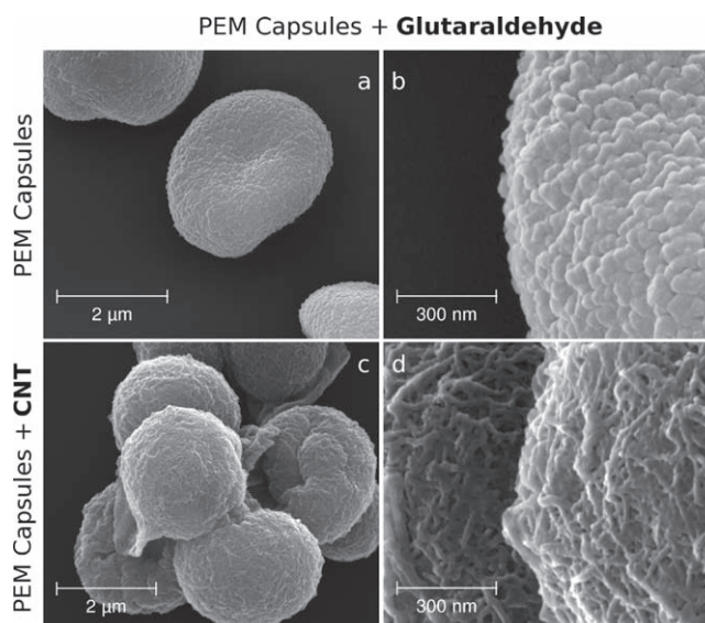
Figure 5. SEM images of microcapsules: a,b) with glutaraldehyde treatment and without carbon nanotubes; c,d) with glutaraldehyde treatment and carbon nanotubes in the microcapsule shells.
