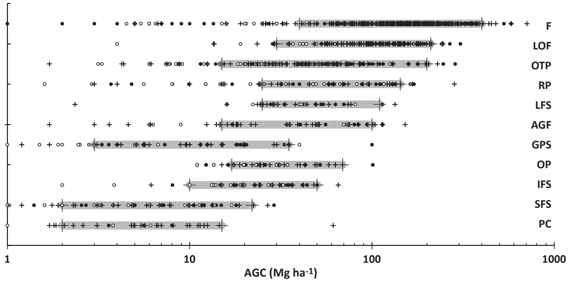
Fig. 1 Summary of above-ground carbon biomass (AGC) values (from Table S1). Open and closed circles are minimum and maximum values of reported ranges, respectively. Crosses refer to reported mean values. The thick line (ending in a cross) is the modified range, defined by the minimum and maximum values reported in Table 3 (also shown in Fig. 2b). Land covers are the following: forest (F); logged over forest (LOF); orchards and tree plantations (OTP); rubber plantations (RP); long-fallow swidden (LFS); nonswidden agroforest (AGF); grassland, pasture, or shrublands (GPS); oil palm plantations (OP); intermediate-fallow swidden (IFS); short-fallow swidden (SFS); and permanent cropland (PC).
