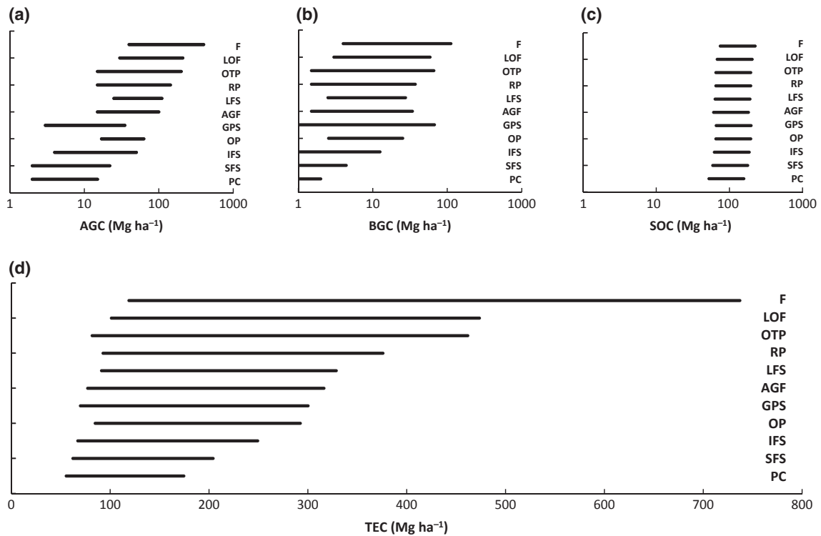
Fig. 2 For the 11 land covers considered in this analysis, plausible ranges of the following: (a) above-ground carbon biomass (AGC); (b) below-ground carbon biomass in vegetation (BGC); (c) soil organic carbon (SOC); and (d) total ecosystem carbon (TEC = AGC + BGC + SOC). Land covers are the following: forest (F); logged over forest (LOF); orchards and tree plantations (OTP); rubber plantations (RP); long-fallow swidden (LFS); nonswidden agroforest (AGF); grassland, pasture, or shrublands (GPS); oil palm plantations (OP); intermediate-fallow swidden (IFS); short-fallow swidden (SFS); and permanent cropland (PC).
